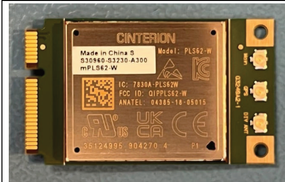
PLS62-W cellular modem
