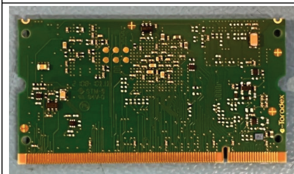
Toradex Colibri iMX7 Dual 1GB Processor module
