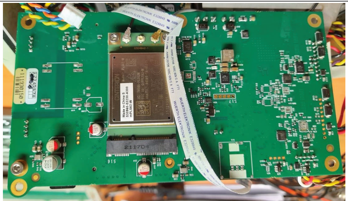
FM3Hub.AAG – Bottom with PLS62-W cellular modem fitted
