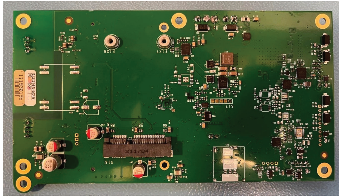
FM3Hub.AAG - Bottom
