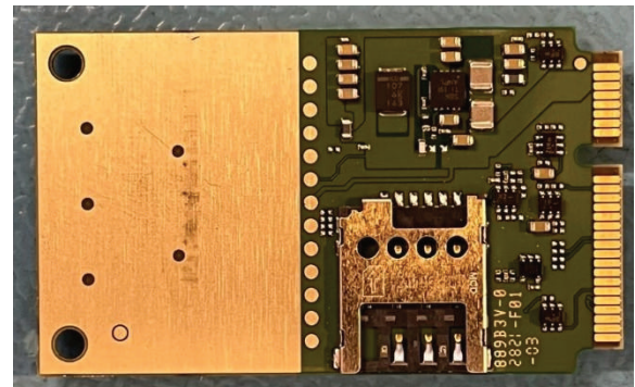
PLS62-W cellular modem
