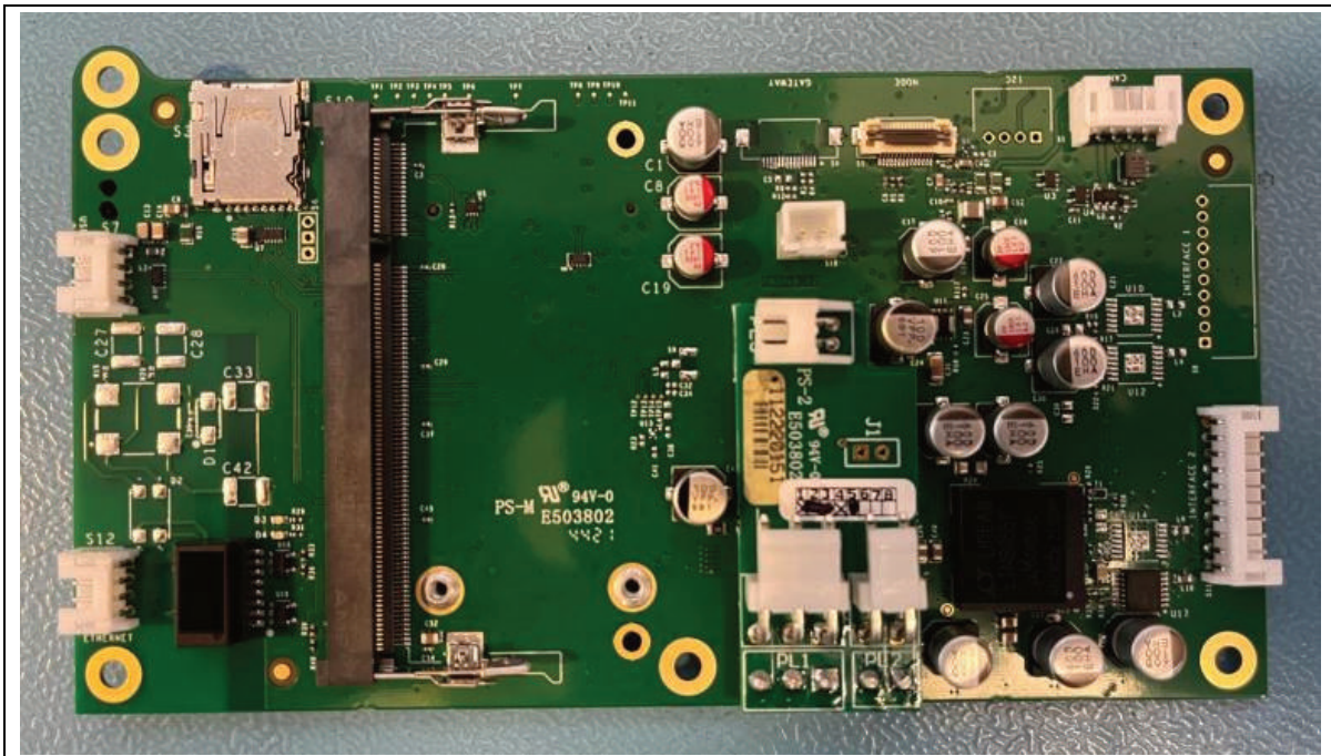
FM3Hub.AAG - Top
