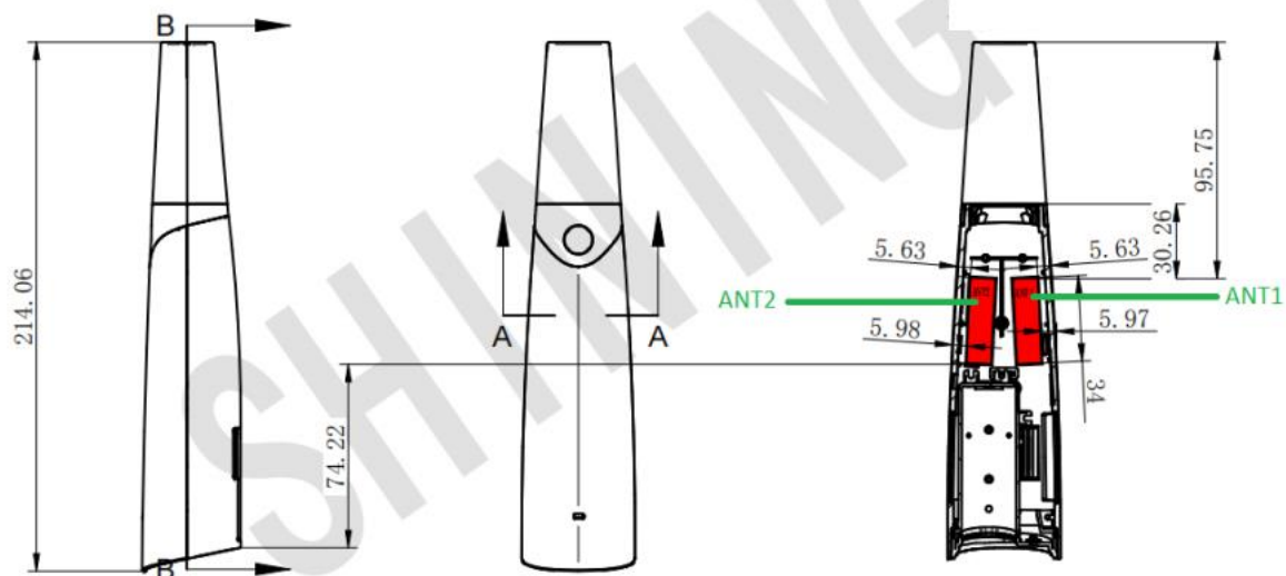
Figure 12.2-1 Antenna Locations
