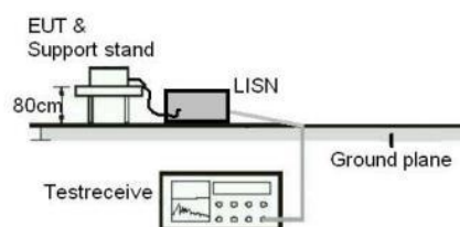
Diagram of Measurement Configuration for Conducted Transmitter Measurement
