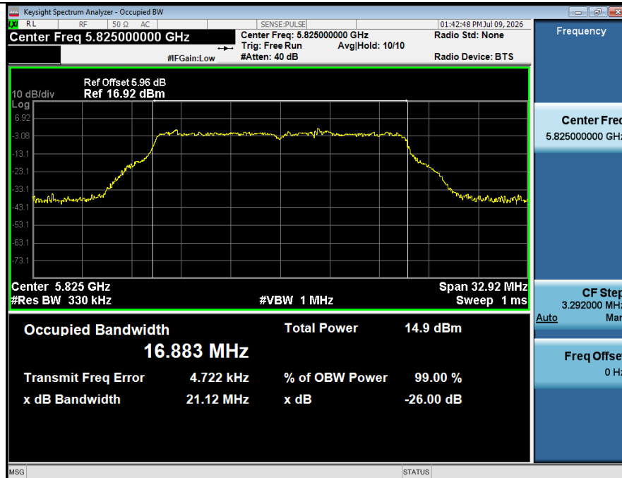
-26BW_NVNT_ANT2_802_11a_5825
