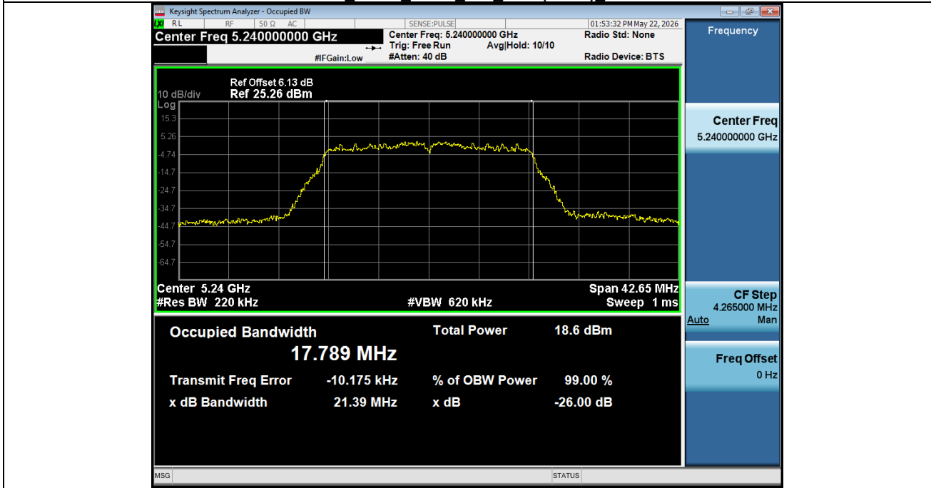
99% OCB NVNT ANT2 802 11ax(HE20) 5240
