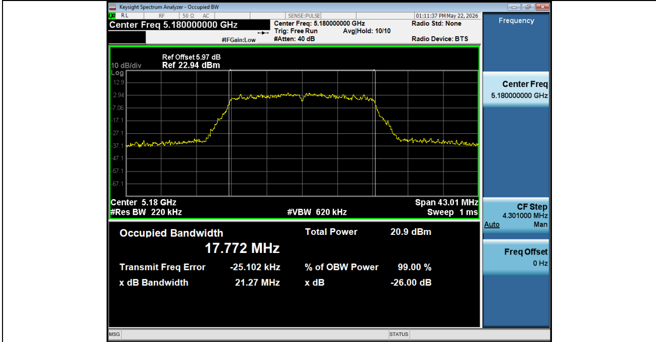
99% OCB_NVNT ANT2 802 11ac(VHT20) 5180
