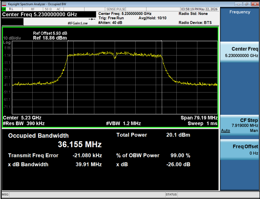
-26BW NVNT ANT2 802 11ac(VHT40) 5230
