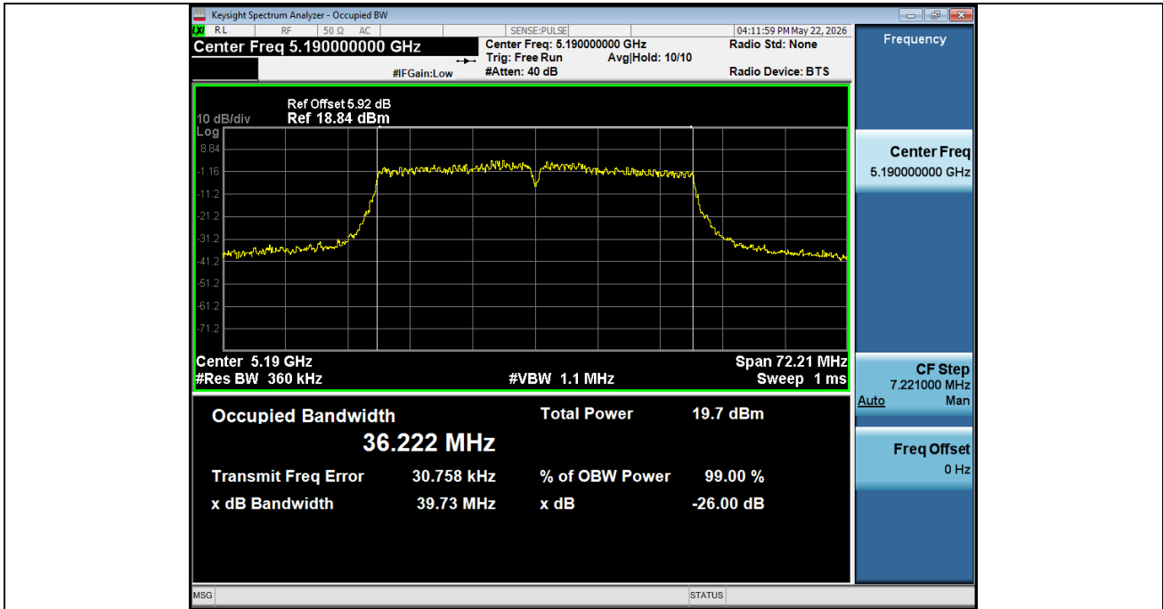
-26BW NVNT ANT2 802 11ac(VHT40) 5190
