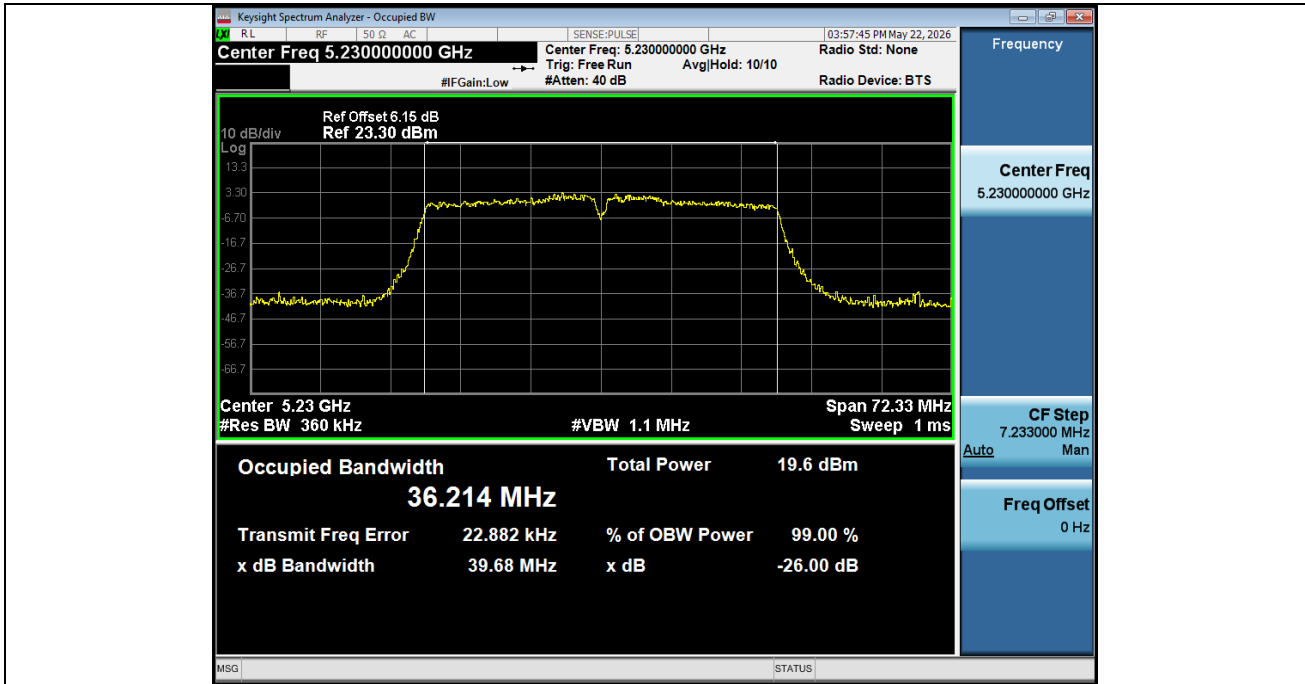
-26BW NVNT ANT1 802 11ac(VHT40) 5230
