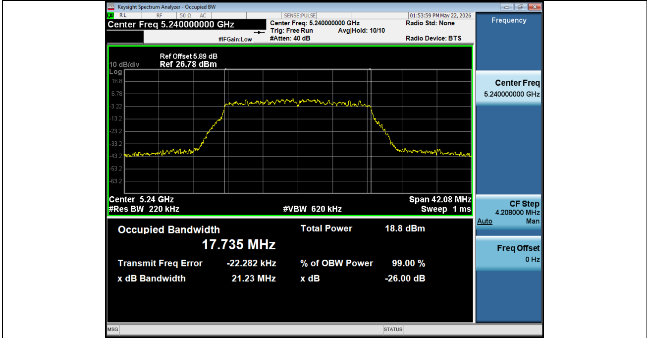
-26BW NVNT ANT2 802 11ax(HE20) 5240
