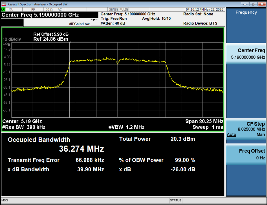
99% OCB NVNT ANT2 802 11ax(HE40) 5190
