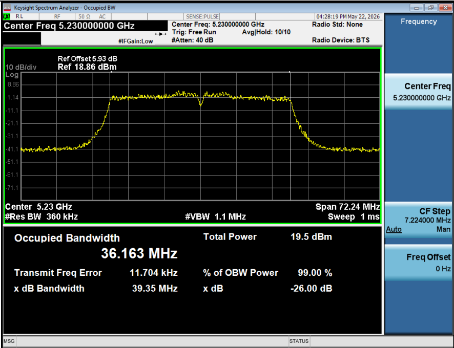
-26BW NVNT ANT2 802 11ax(HE40) 5230
