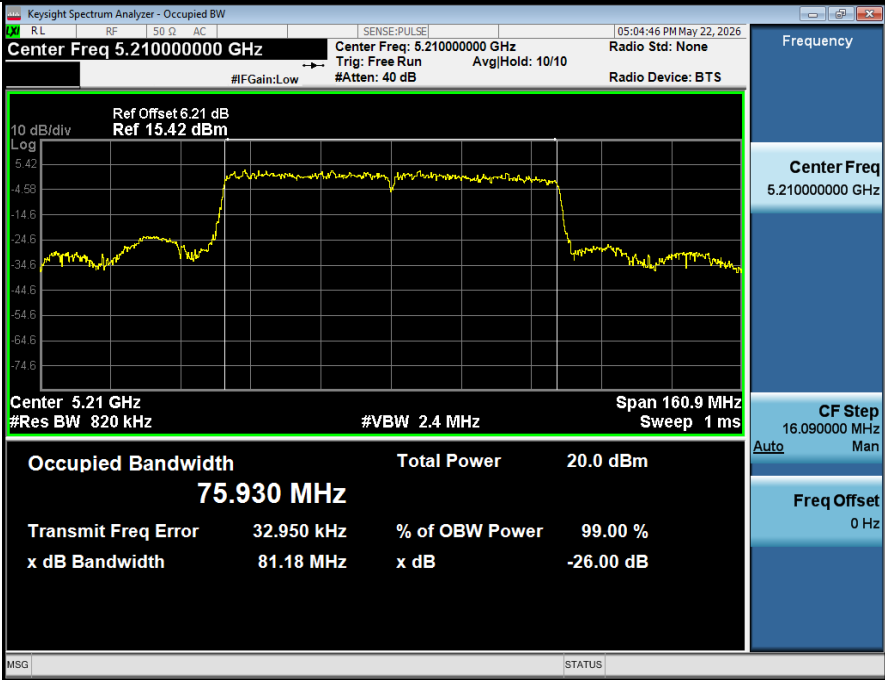
-26BW NVNT ANT2 802 11ax(HE80) 5210
