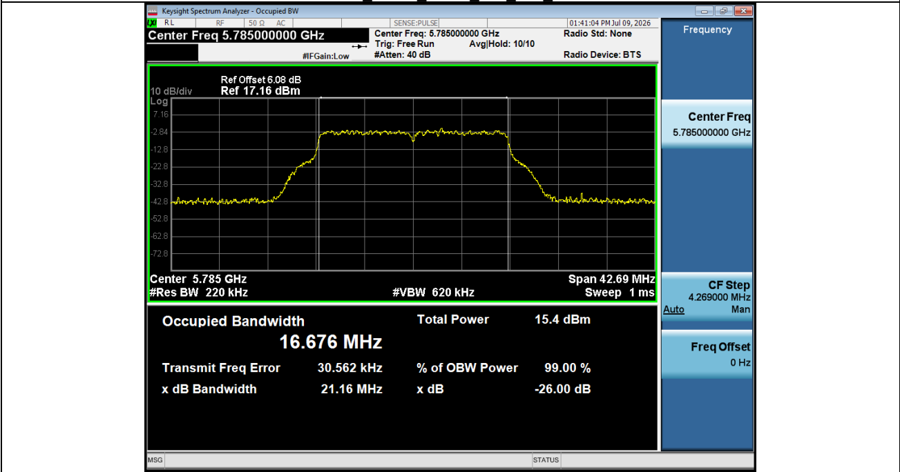
-26BW NVNT ANT2 802 11a 5785
