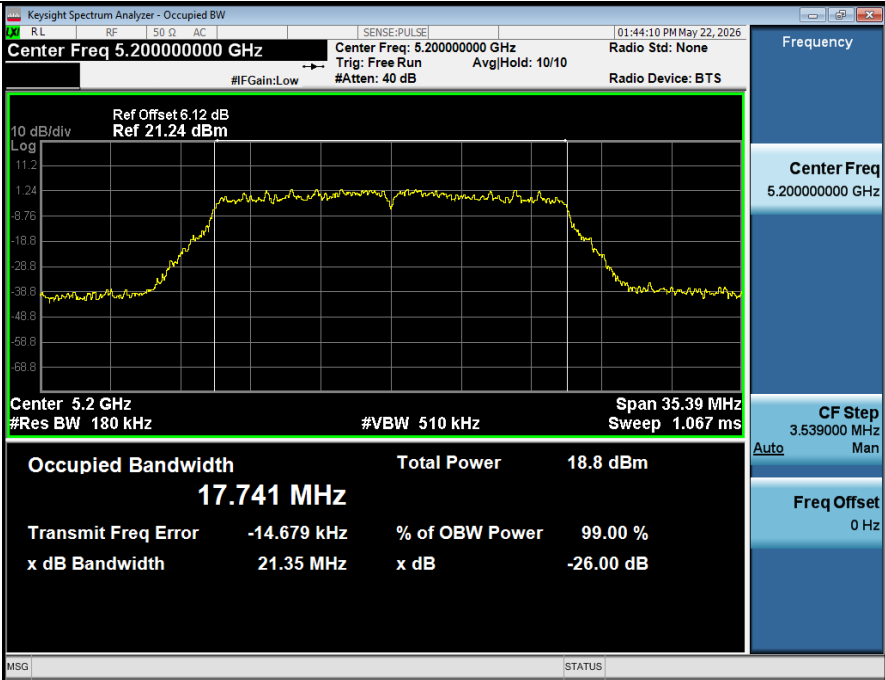
-26BW NVNT ANT1 802 11ax(HE20) 5200
