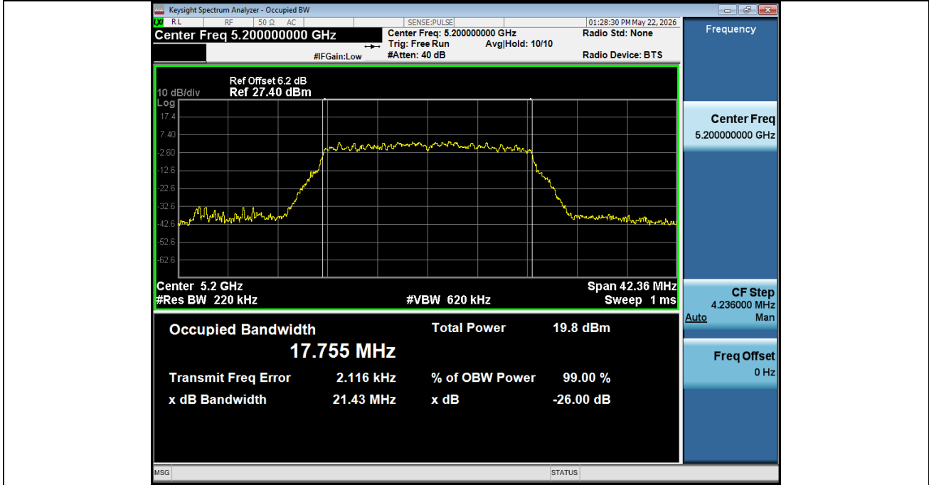
-26BW NVNT ANT2 802 11ac(VHT20) 5200
