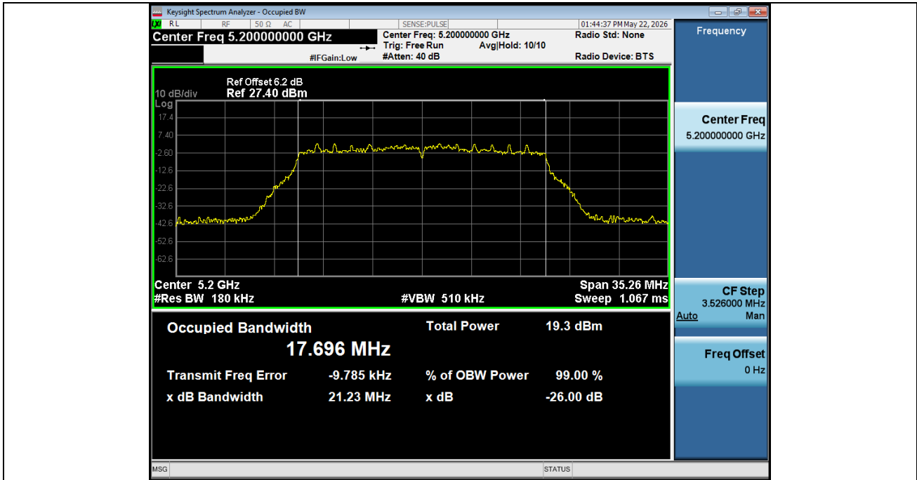
-26BW NVNT ANT2 802 11ax(HE20) 5200
