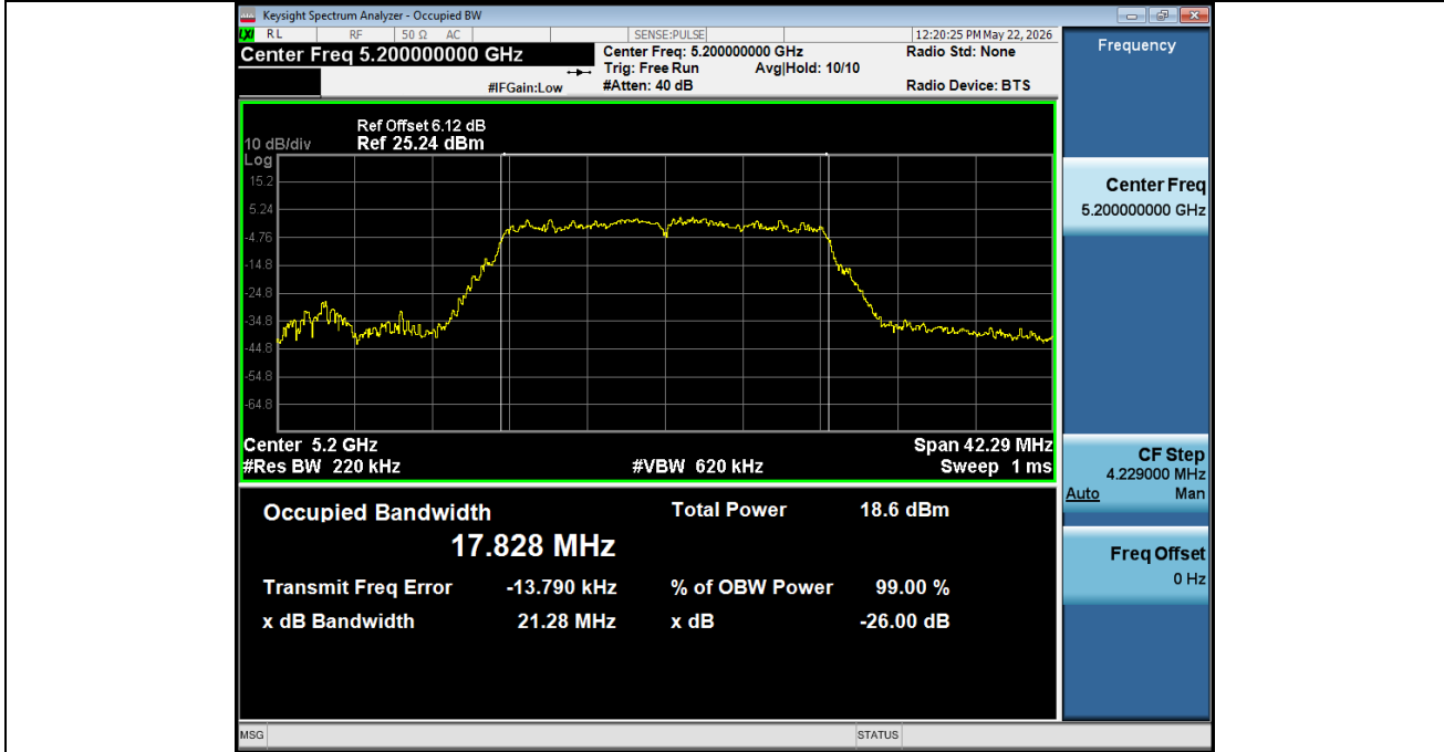
99% OCB NVNT ANT2 802 11n(HT20) 5200
