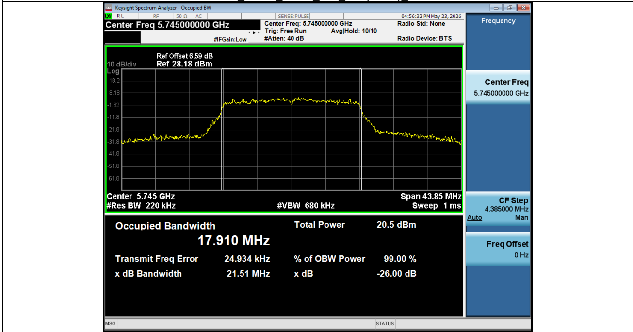
99% OCB NVNT ANT2 802 11n(HT20) 5745
