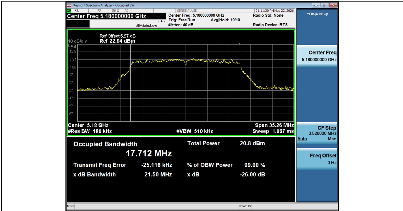
-26BW NVNT ANT1 802 11ac(VHT20) 5180
