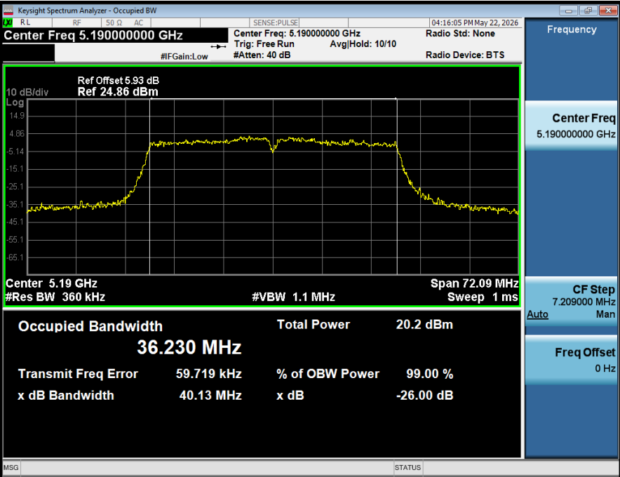
-26BW NVNT ANT1 802 11ax(HE40) 5190
