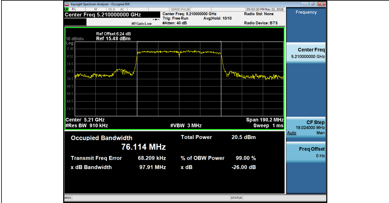
99%_OCB_NVNT_ANT2_802_11ac(VHT80)_5210
