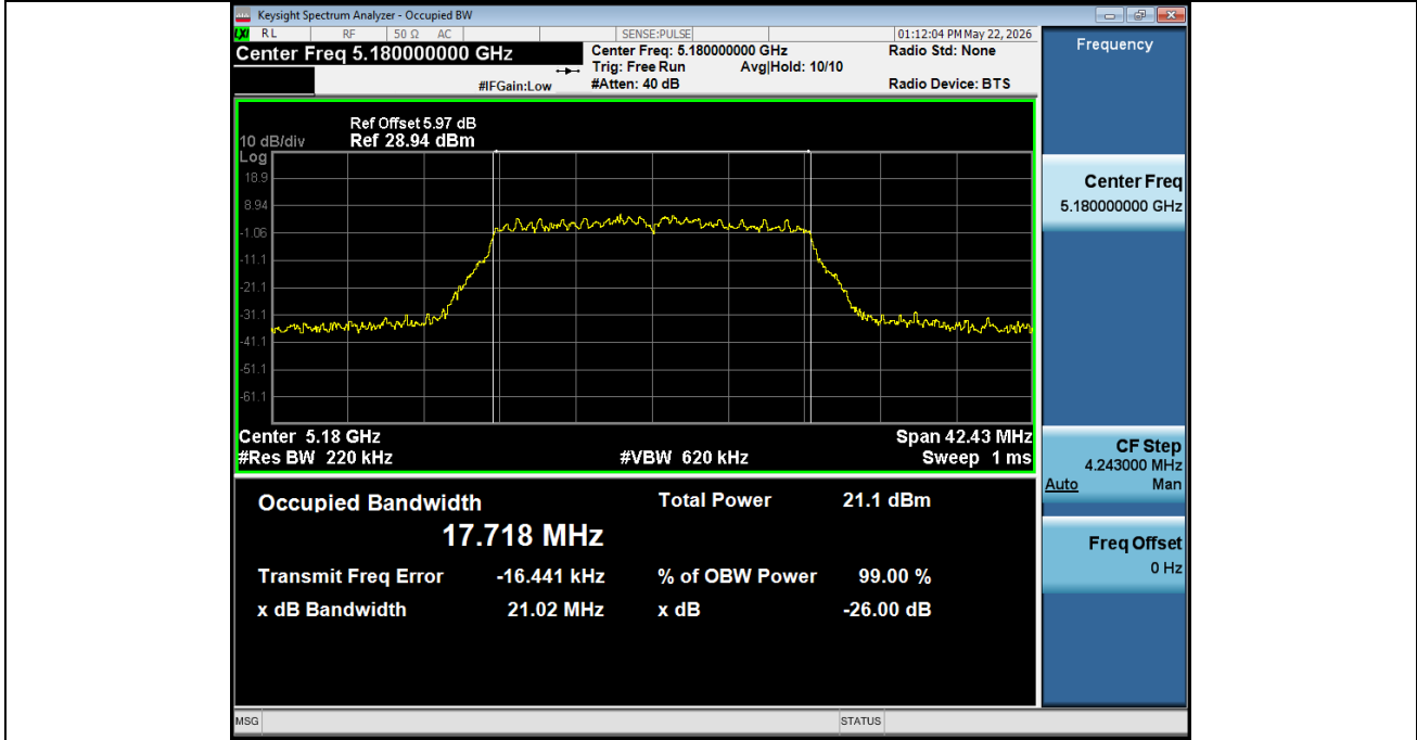
-26BW NVNT ANT2 802 11ac(VHT20) 5180
