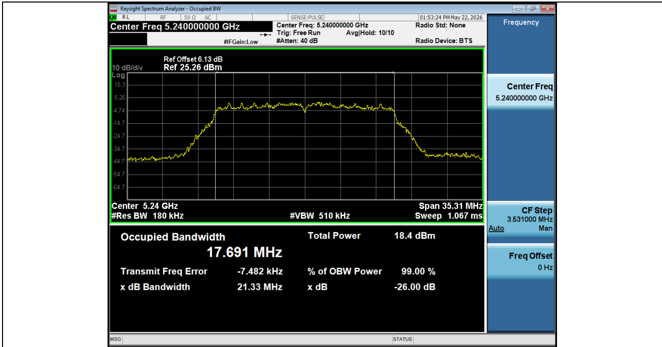
-26BW NVNT ANT1 802 11ax(HE20) 5240
