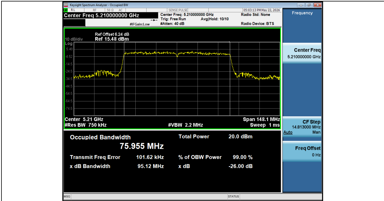
-26BW NVNT ANT1 802 11ac(VHT80) 5210
