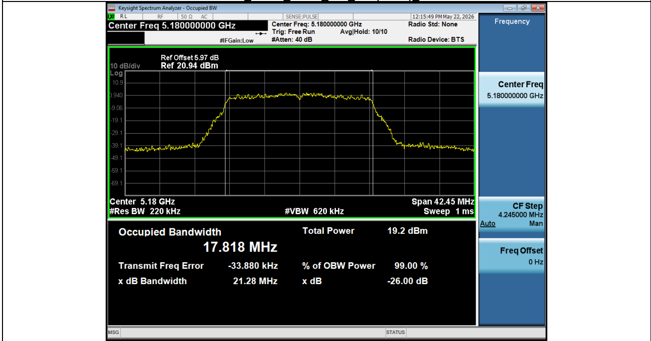
99% OCB NVNT ANT2 802 11n(HT20) 5180
