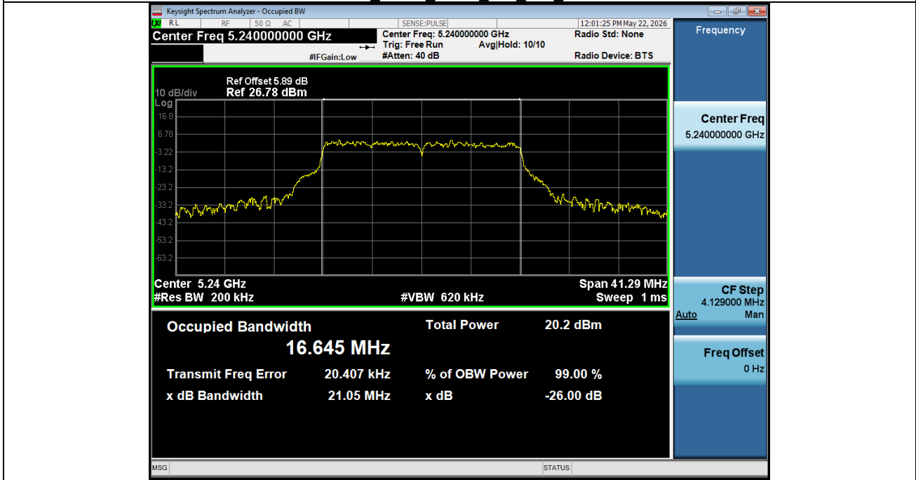
-26BW NVNT ANT2 802 11a 5240
