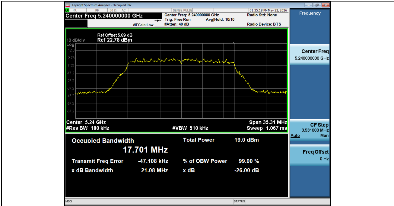
-26BW NVNT ANT2 802 11ac(VHT20) 5240
