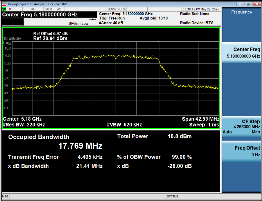
99% OCB NVNT ANT2 802 11ax(HE20) 5180
