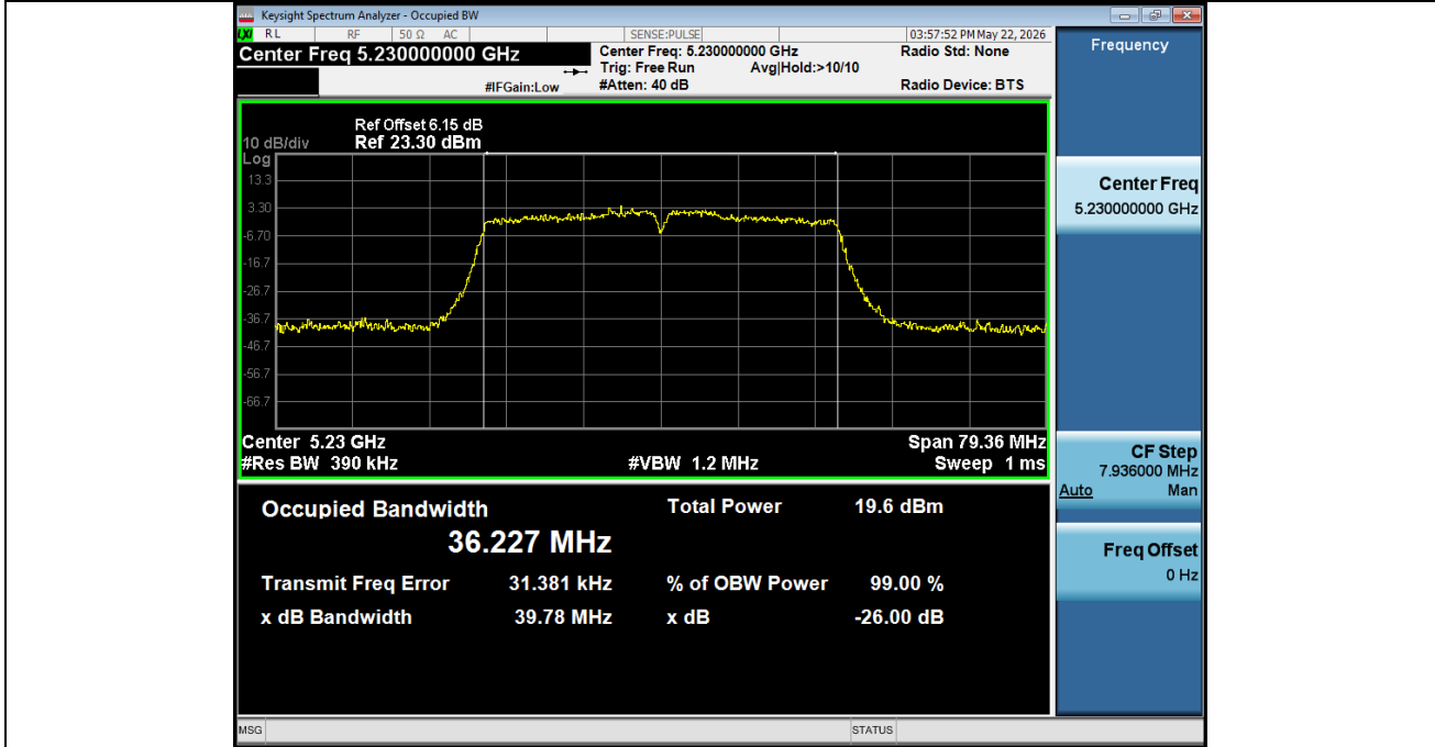
99%_OCB_NVNT_ANT2_802_11ac(VHT40)_5230
