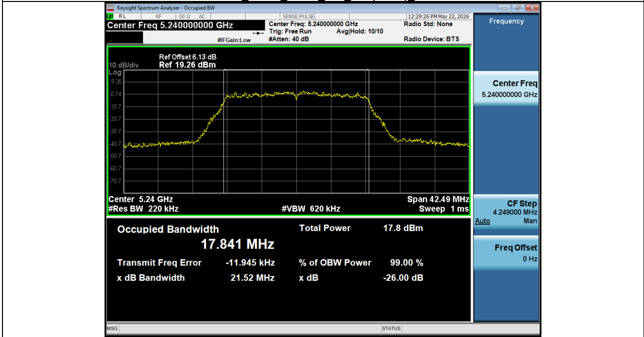
99% OCB NVNT ANT2 802 11n(HT20) 5240
