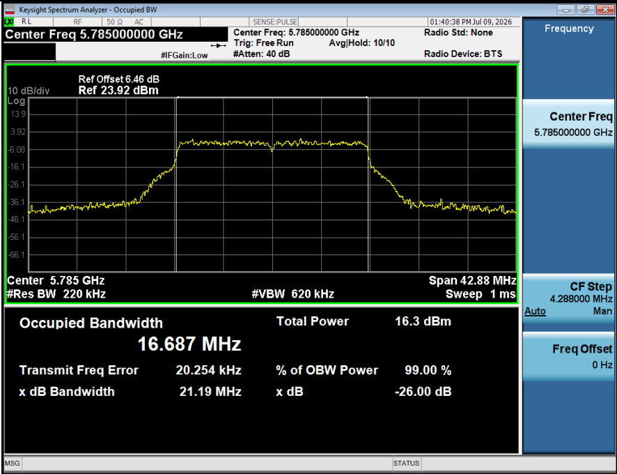
99%_OCB_NVNT_ANT2_802_11a_5785
