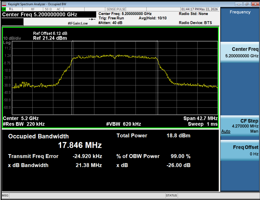
99% OCB NVNT ANT2 802 11ax(HE20) 5200
