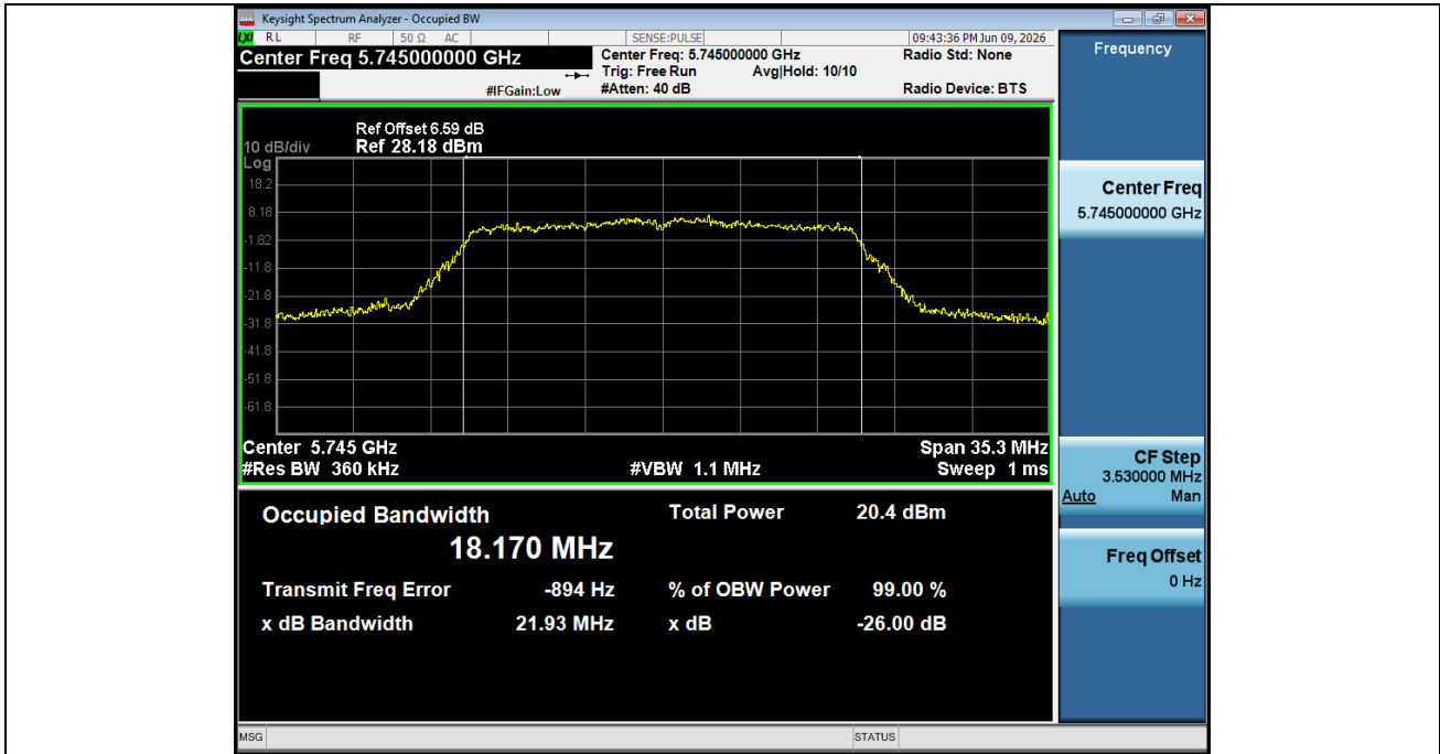
-26BW NVNT ANT1 802 11ac(VHT20) 5745
