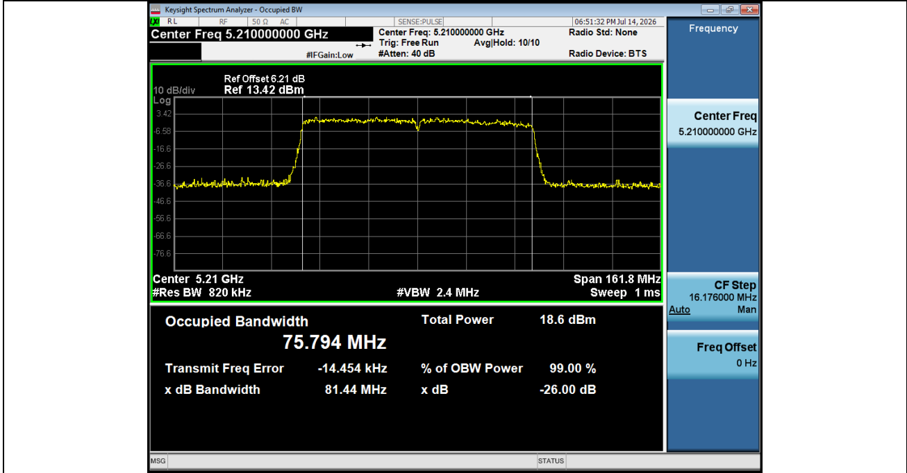
-26BW NVNT ANT2 802 11ac(VHT80) 5210
