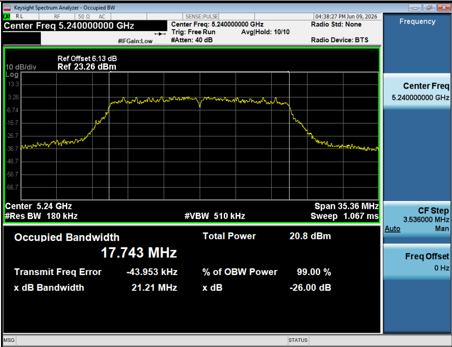
-26BW NVNT ANT1 802 11ac(VHT20) 5240
