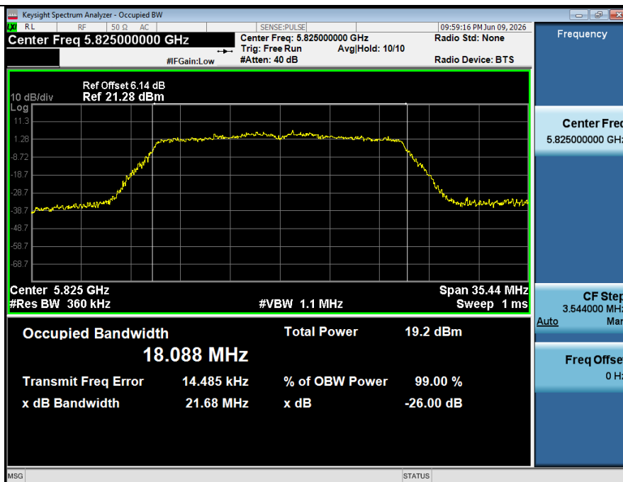
-26BW_NVNT_ANT1_802_11n(HT20)_5825
