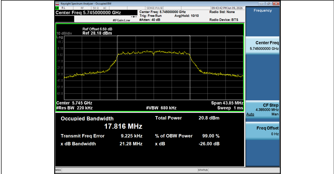
99% OCB NVNT ANT2 802 11ac(VHT20) 5745
