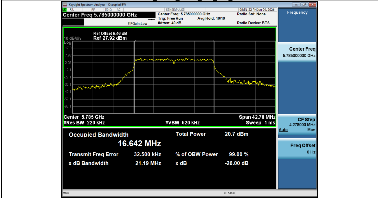
99%_OCB_NVNT_ANT2_802_11a_5785
