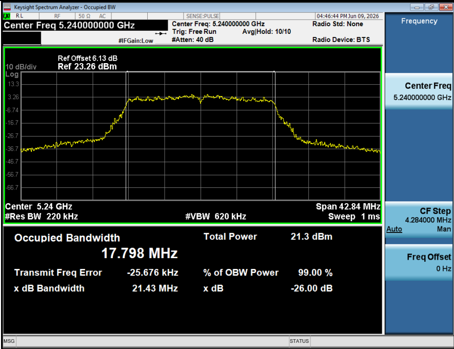
99% OCB NVNT ANT2 802 11ax(HE20) 5240
