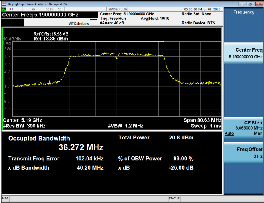
99%_OCB_NVNT_ANT2_802_11ac(VHT40)_5190
