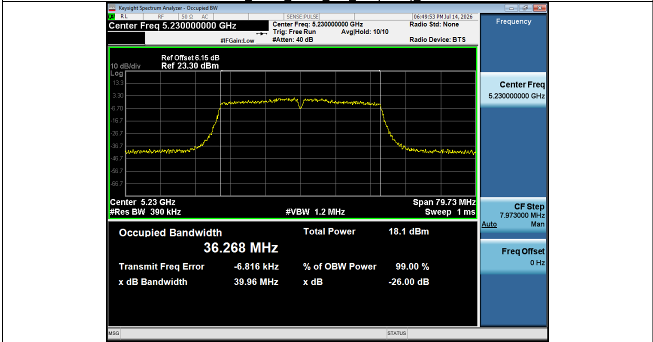
99% OCB NVNT ANT2 802 11n(HT40) 5230
