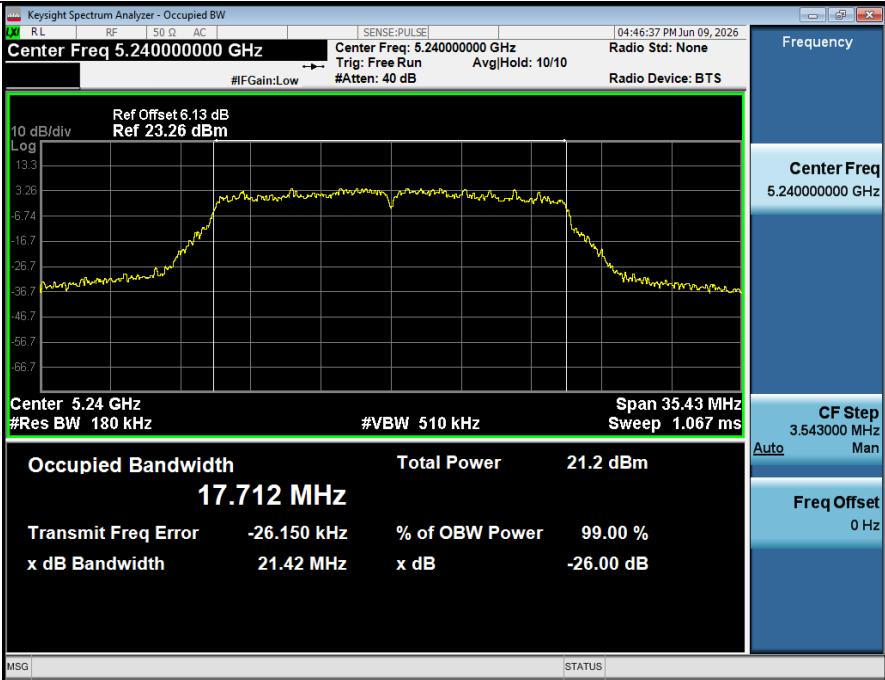
-26BW NVNT ANT1 802 11ax(HE20) 5240
