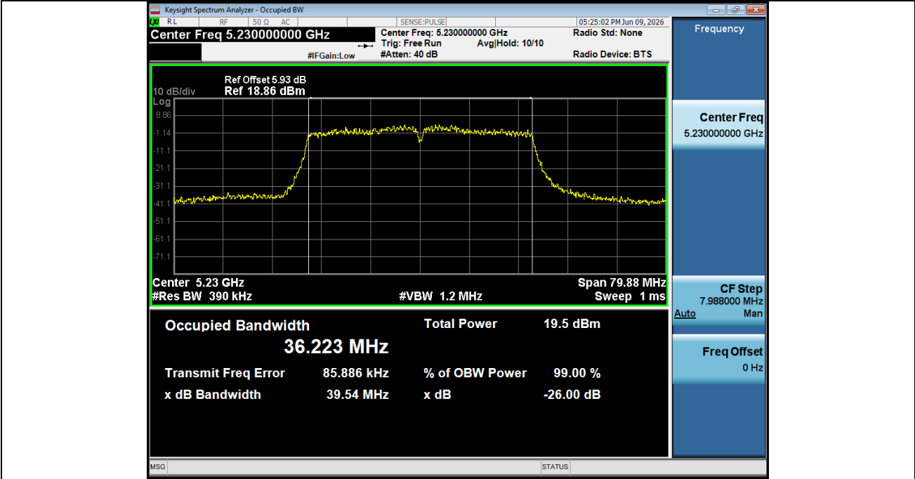
-26BW NVNT ANT2 802 11ax(HE40) 5230
