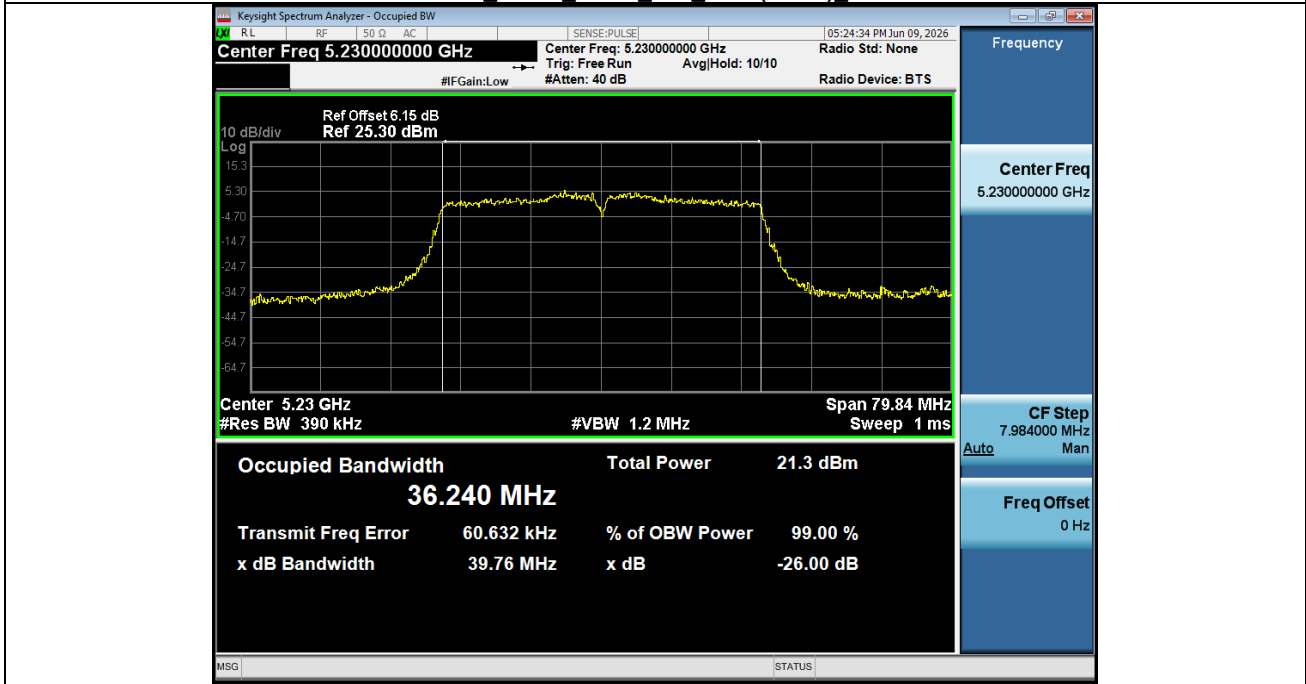
99% OCB NVNT ANT2 802 11ax(HE40) 5230
