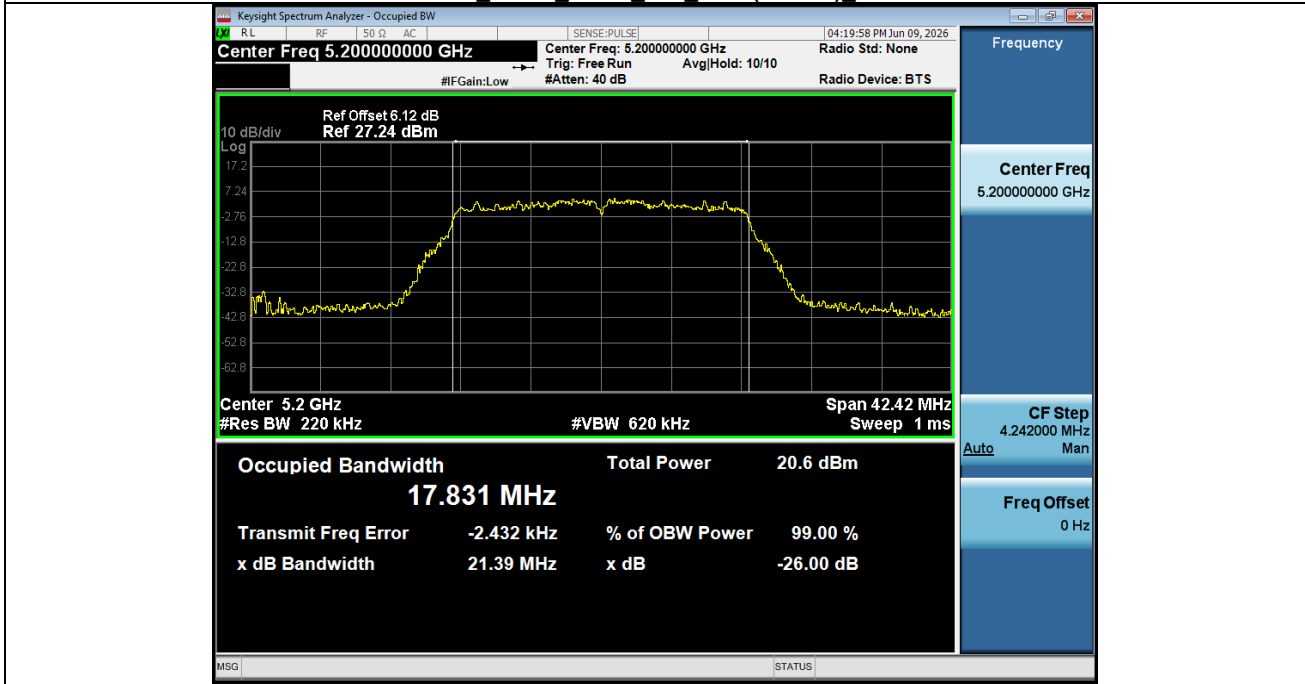
99%_OCB_NVNT_ANT2_802_11ac(VHT20)_5200
