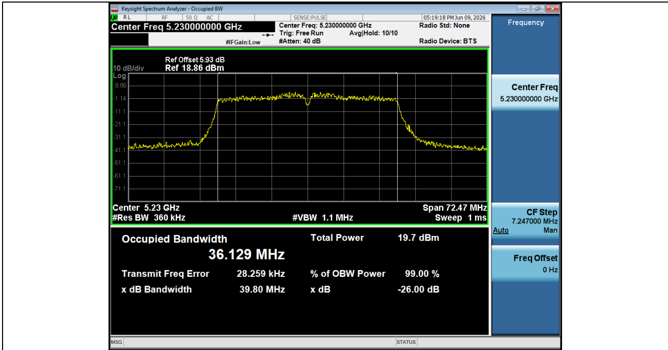
-26BW NVNT ANT2 802 11ac(VHT40) 5230
