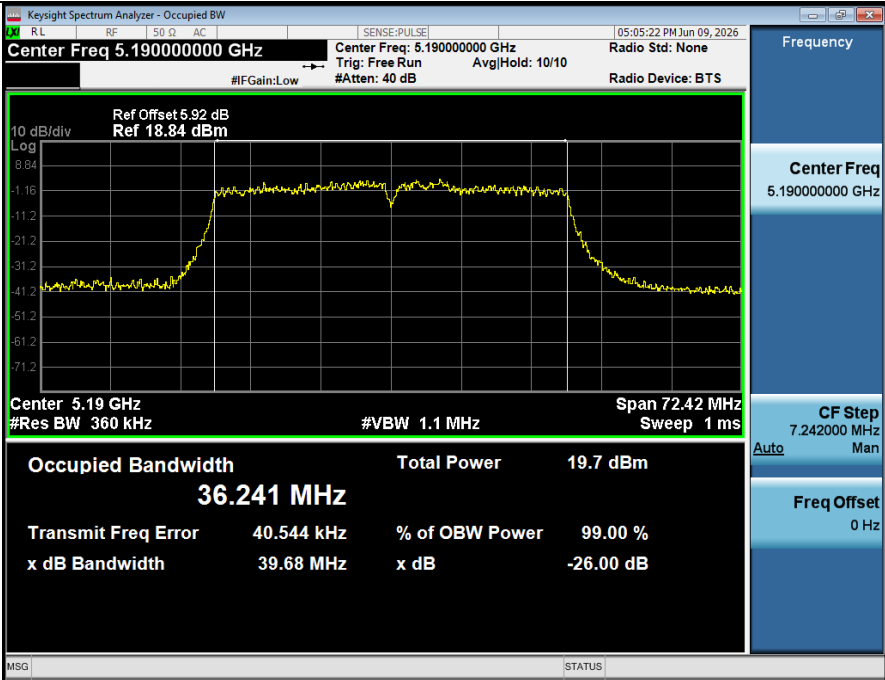
-26BW NVNT ANT2 802 11ac(VHT40) 5190
