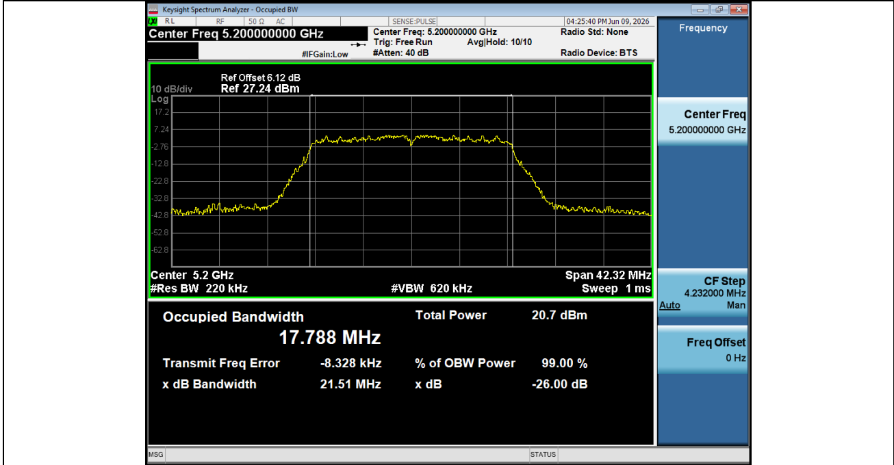
99% OCB NVNT ANT2 802 11ax(HE20) 5200
