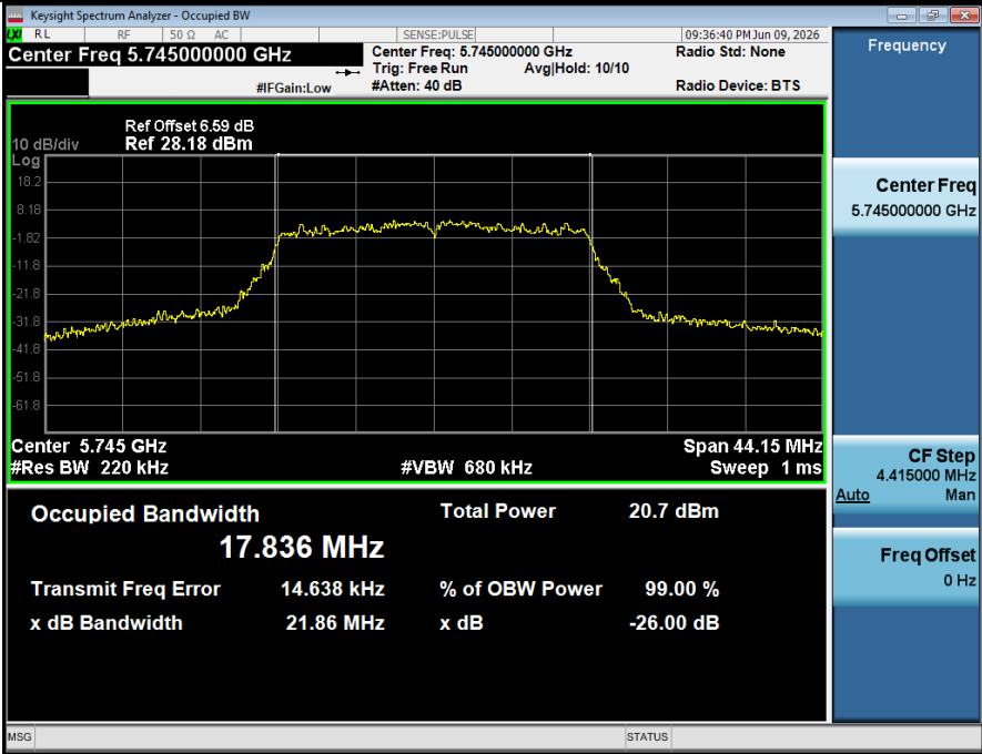
99% OCB NVNT ANT2 802 11n(HT20) 5745
