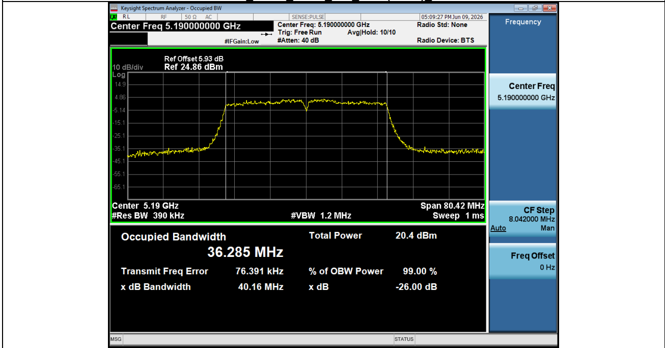
99% OCB NVNT ANT2 802 11ax(HE40) 5190
