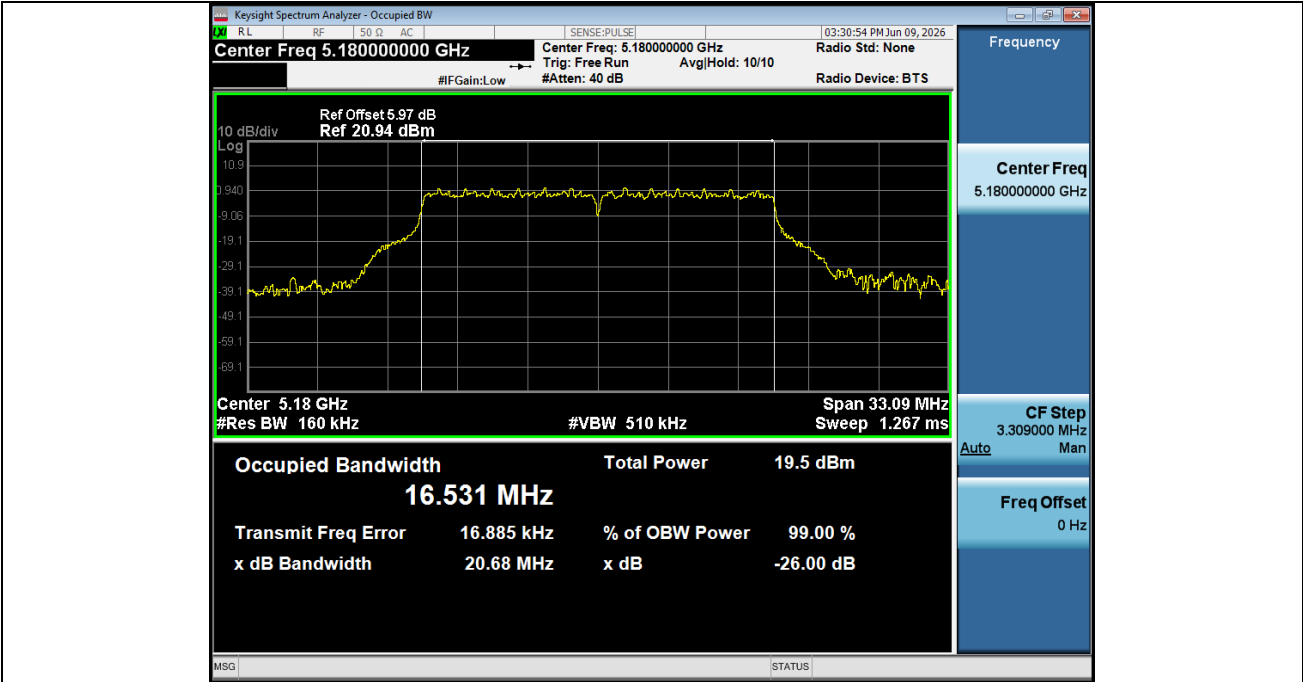
-26BW NVNT ANT2 802 11a 5180
