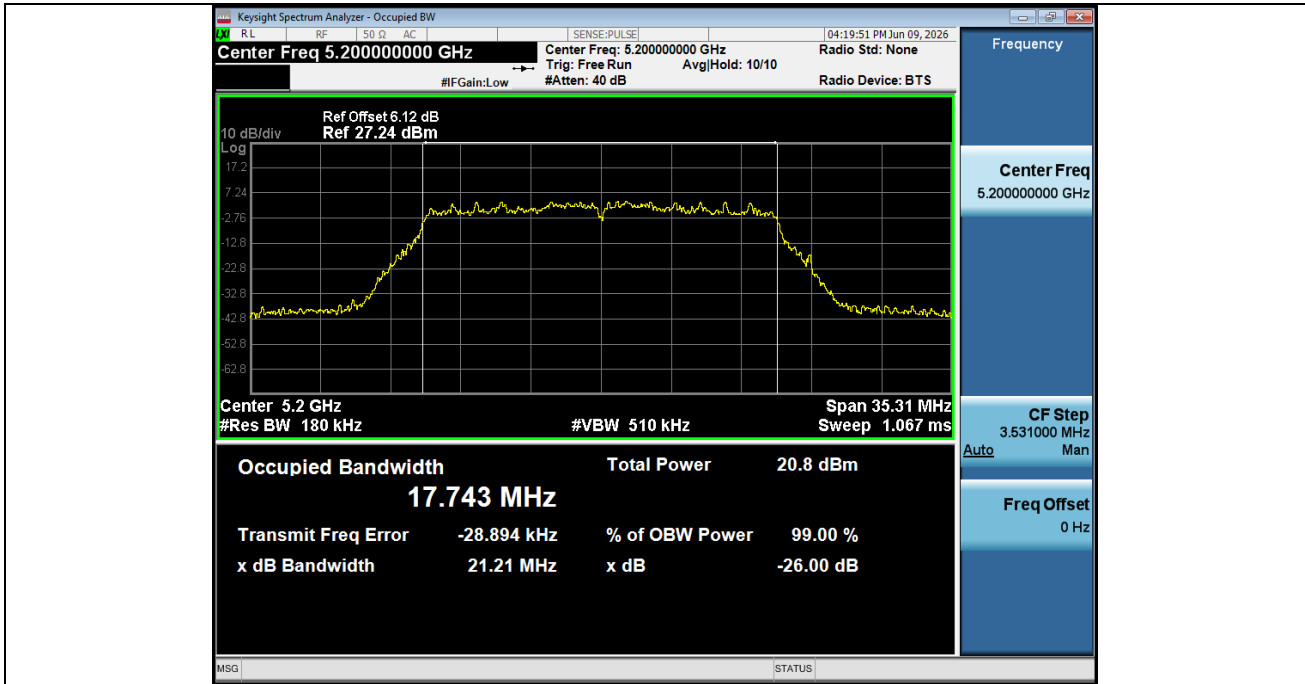
-26BW NVNT ANT1 802 11ac(VHT20) 5200
