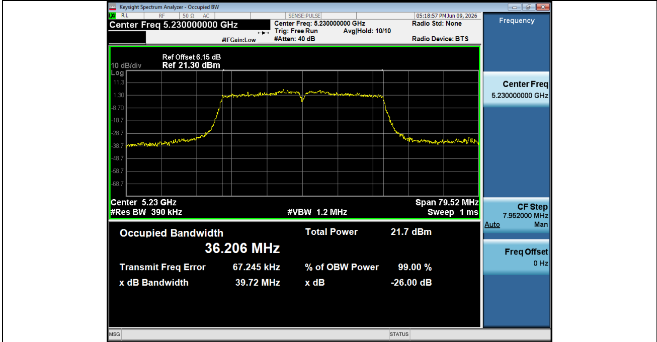
99%_OCB_NVNT_ANT2_802_11ac(VHT40)_5230
