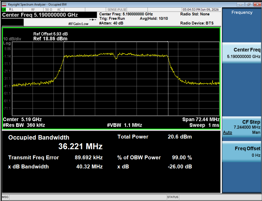
-26BW NVNT ANT1 802 11ac(VHT40) 5190
