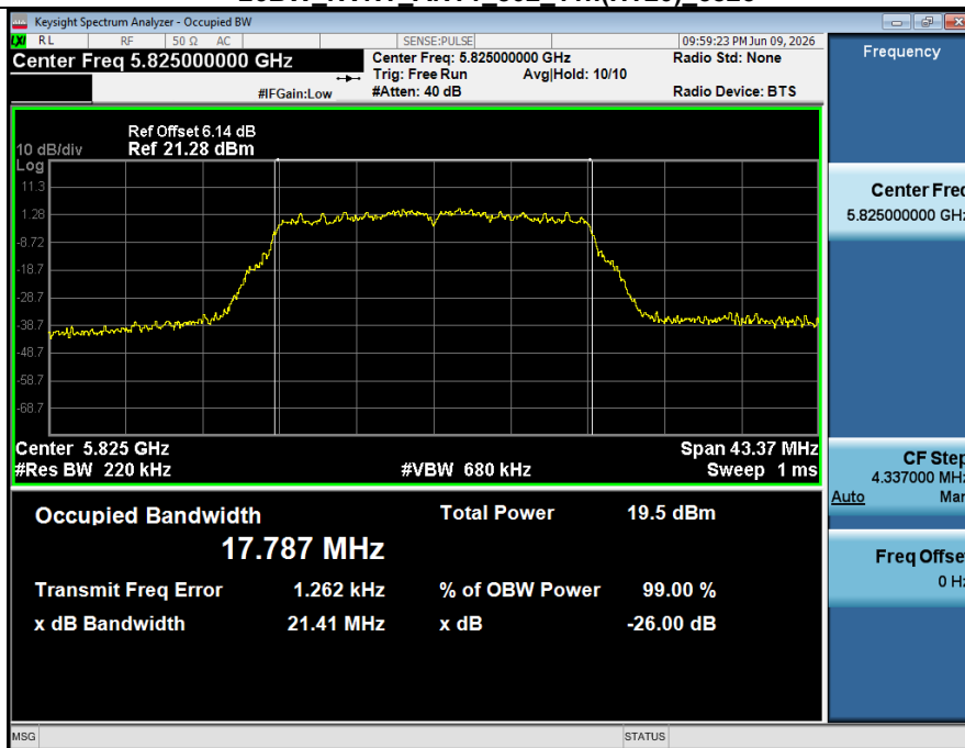
99% OCB NVNT ANT2 802 11n(HT20) 5825
