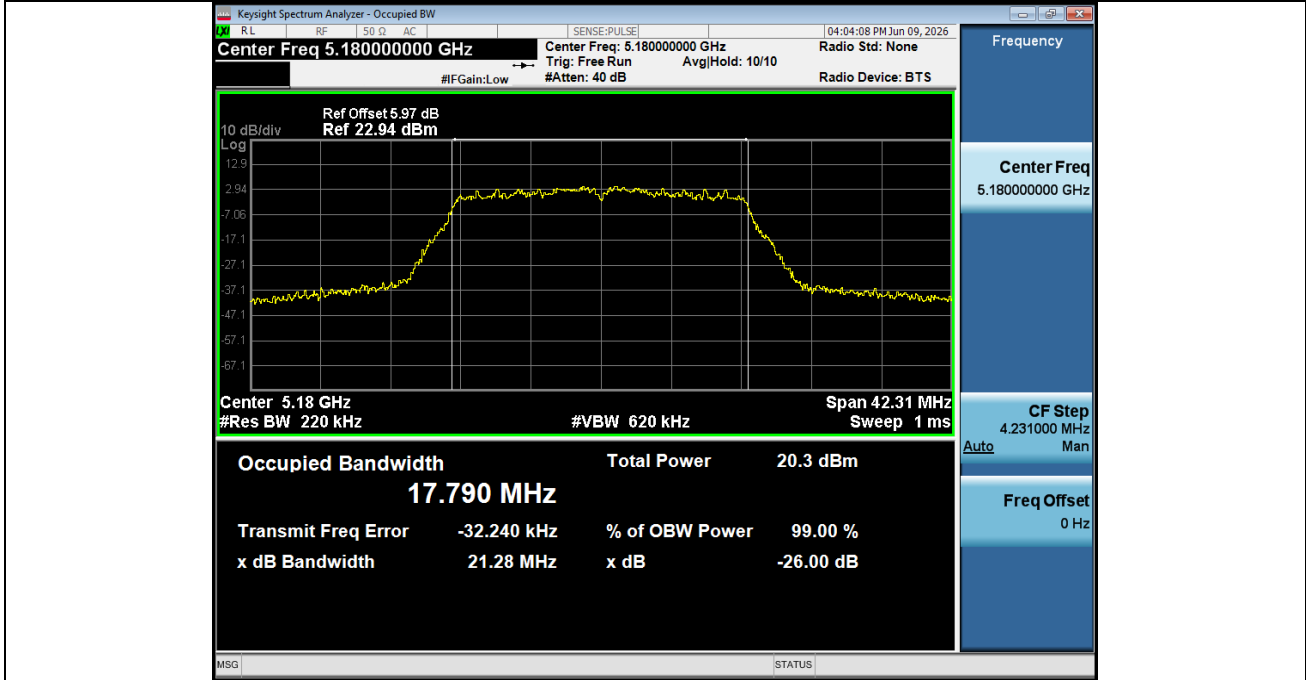
99%_OCB_NVNT_ANT2_802_11ac(VHT20)_5180
