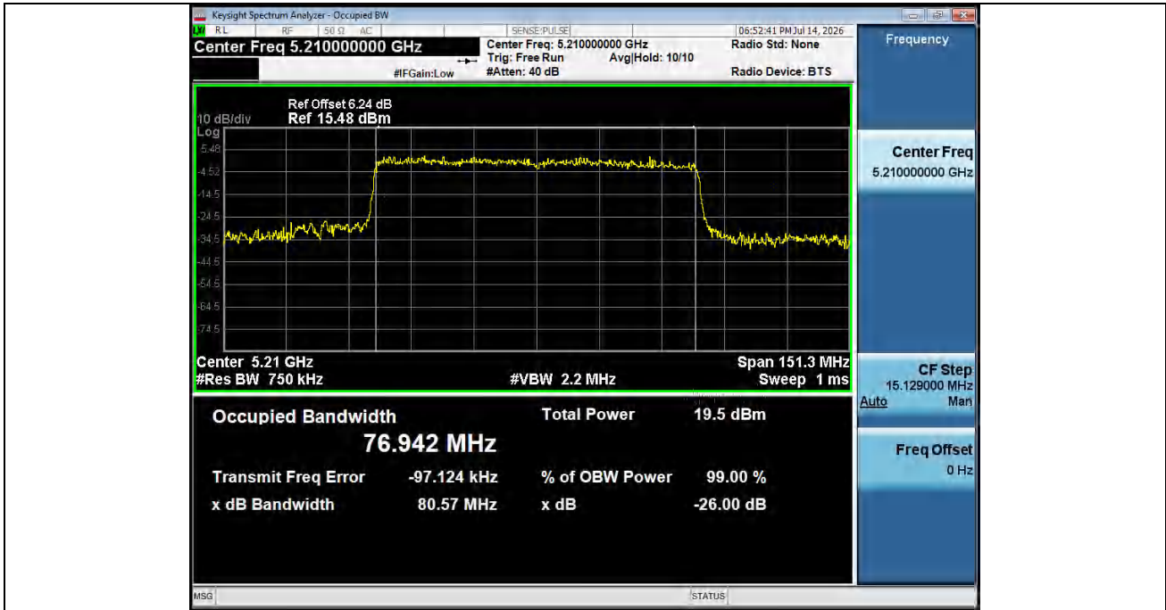
-26BW_NVNT_ANT1_802_11ax(HE80)_5210
