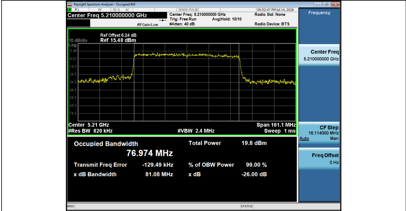
99%_OCB_NVNT_ANT2_802_11ax(HE80)_5210
