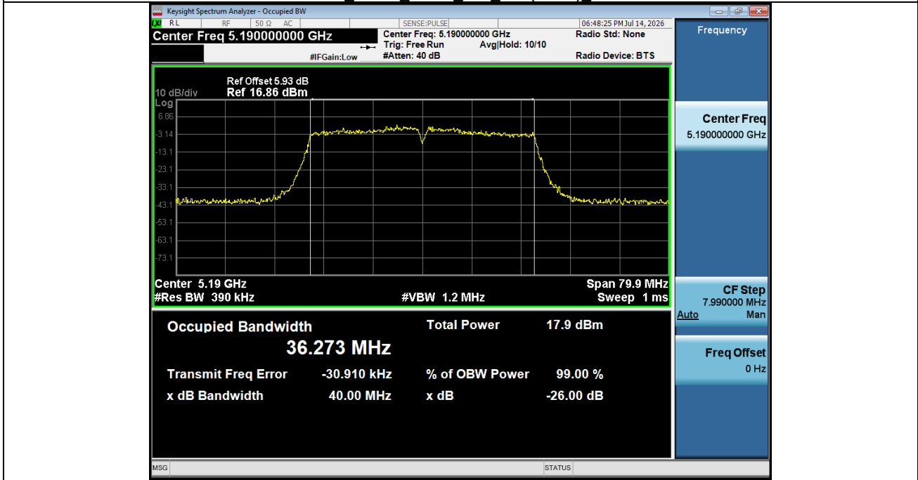
99% OCB NVNT ANT2 802 11n(HT40) 5190
