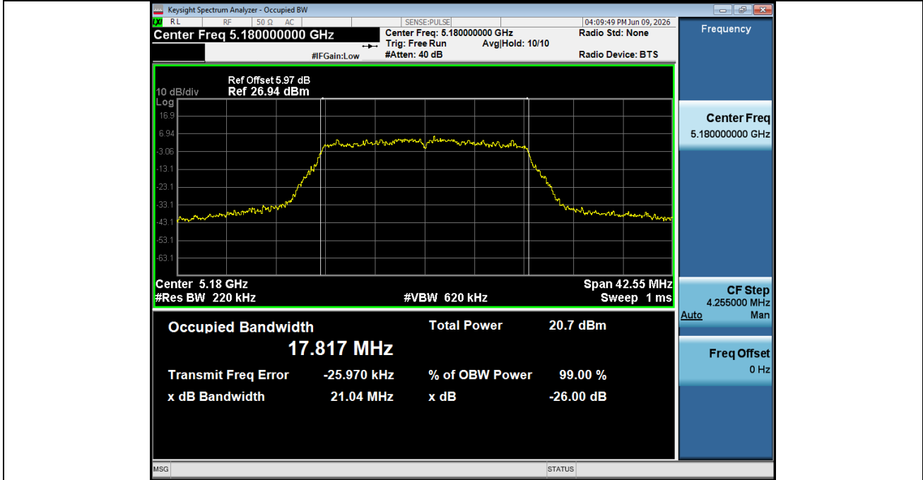
99% OCB NVNT ANT2 802 11ax(HE20) 5180
