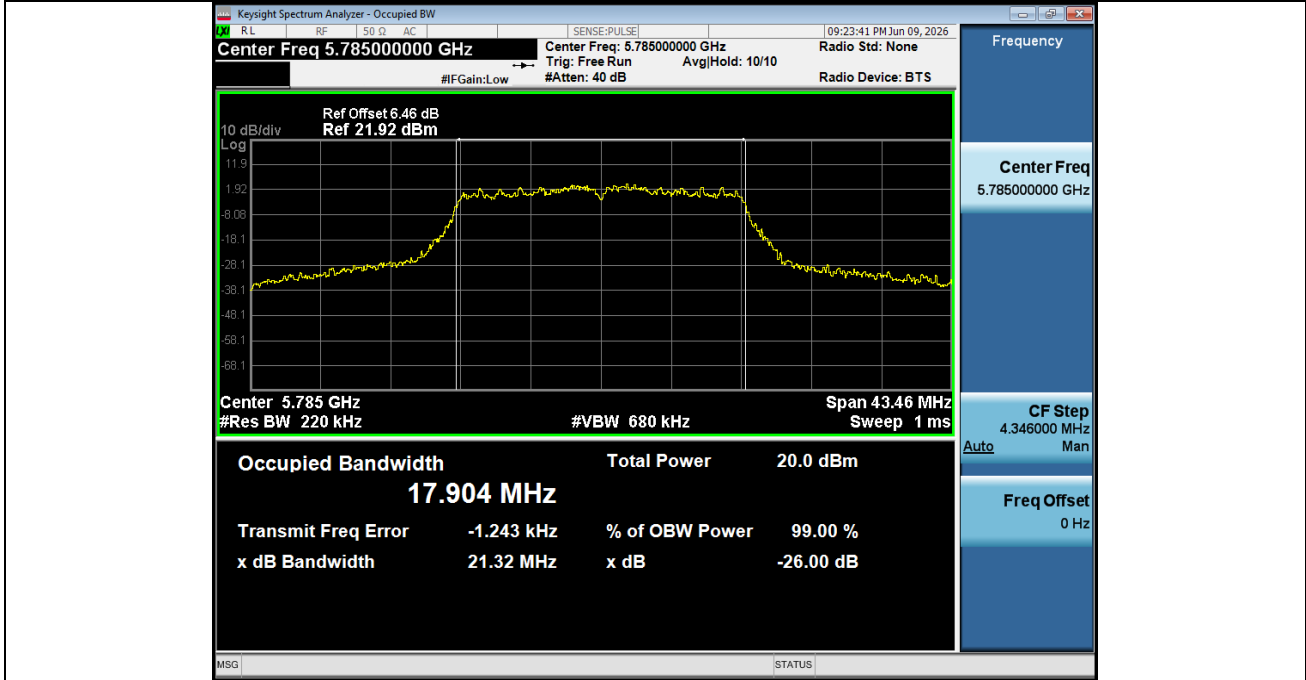
99% OCB NVNT ANT2 802 11ac(VHT20) 5785
