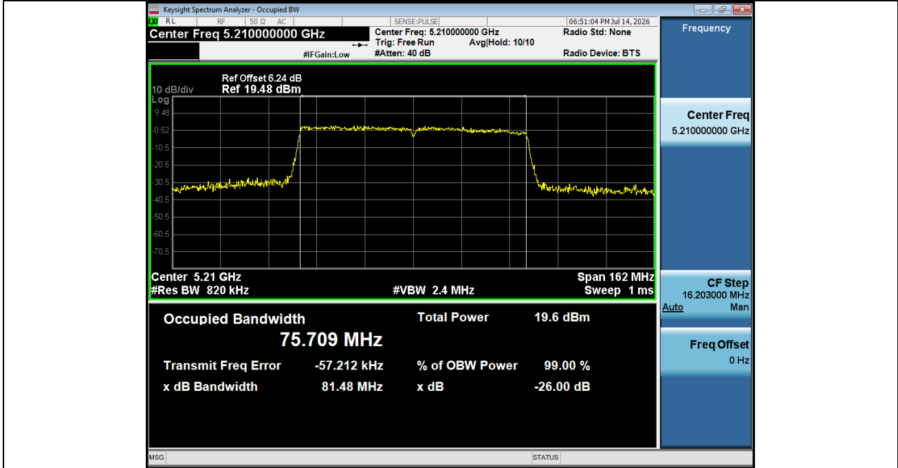
99%_OCB_NVNT_ANT2_802_11ac(VHT80)_5210
