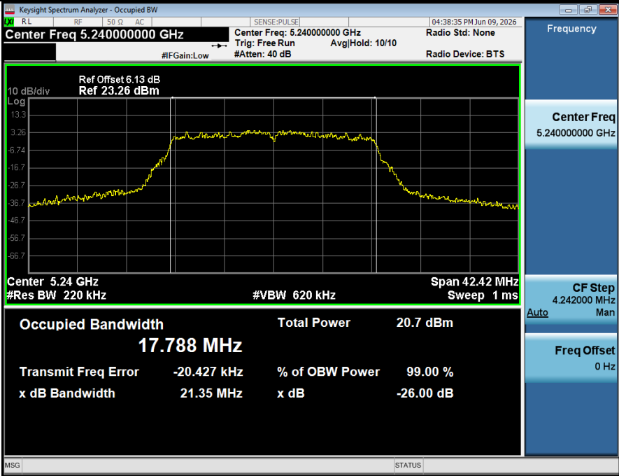
99%_OCB_NVNT_ANT2_802_11ac(VHT20)_5240
