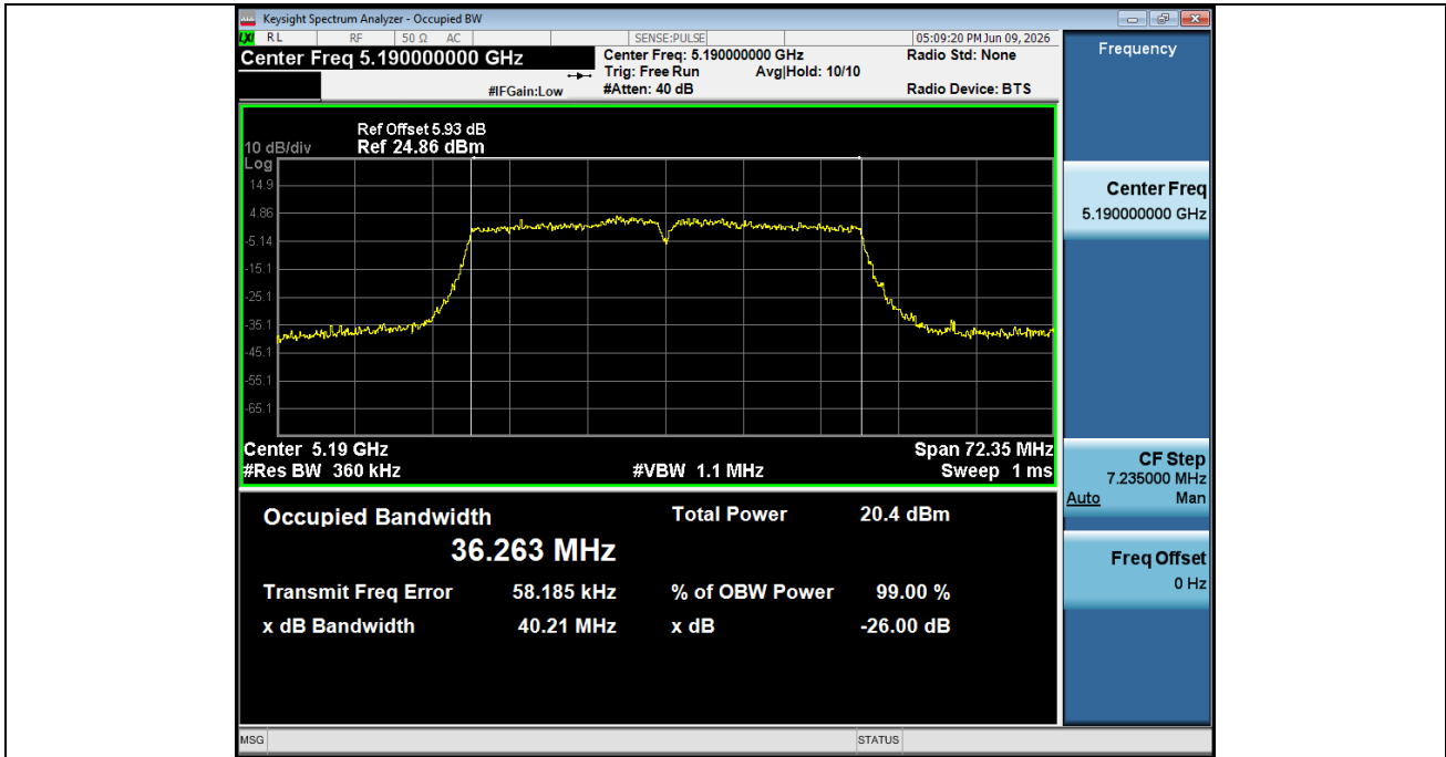
-26BW NVNT ANT1 802 11ax(HE40) 5190
