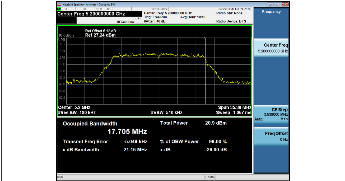
-26BW NVNT ANT1 802 11ax(HE20) 5200
