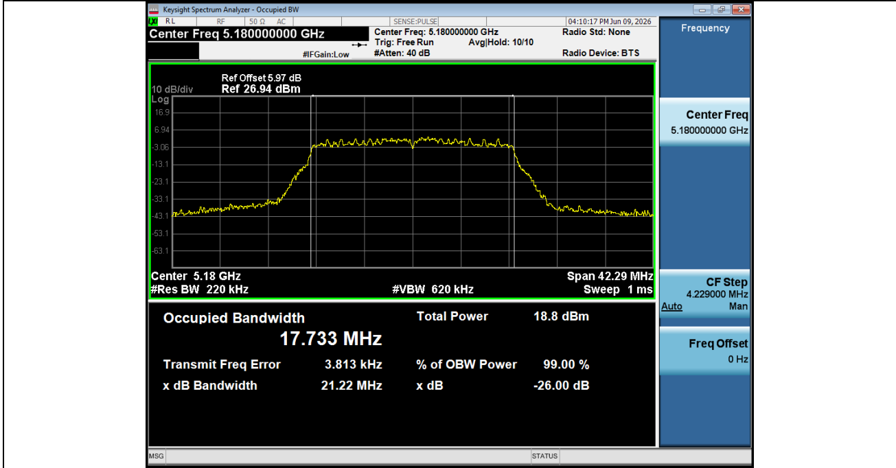
-26BW NVNT ANT2 802 11ax(HE20) 5180
