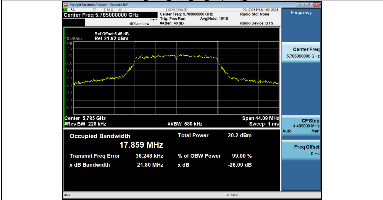
99% OCB NVNT ANT2 802 11n(HT20) 5785
