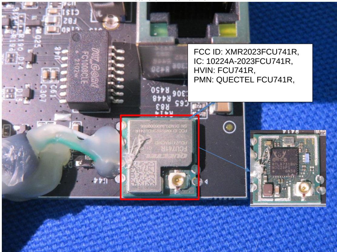
Picture 6 -The certified Module
