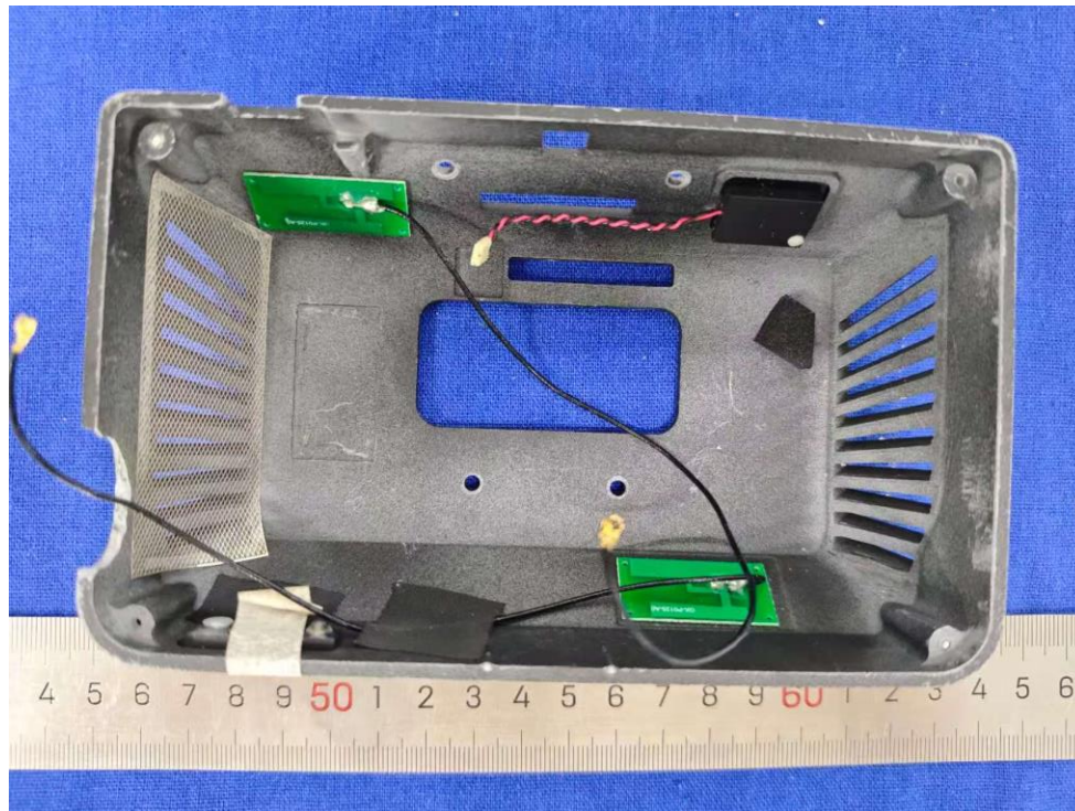
Product: 3D Scanner Model: FreeScan Omni
