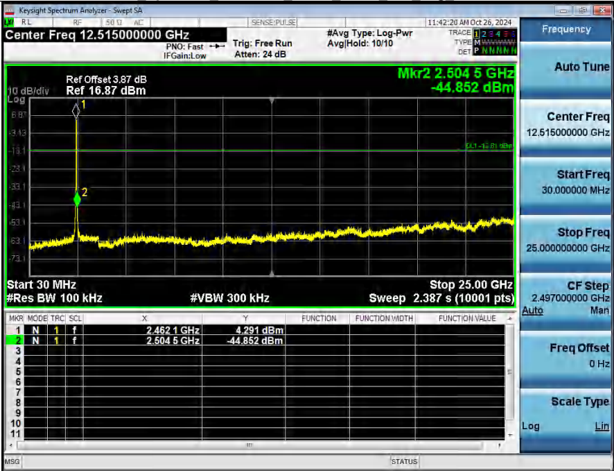
2_Spurious_Emission_NVNT_ANT1_802_11g_2462
