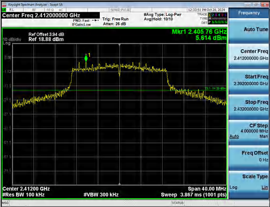
1 Reference_Level_NVNT_ANT2_802_11n(HT20)_2412
