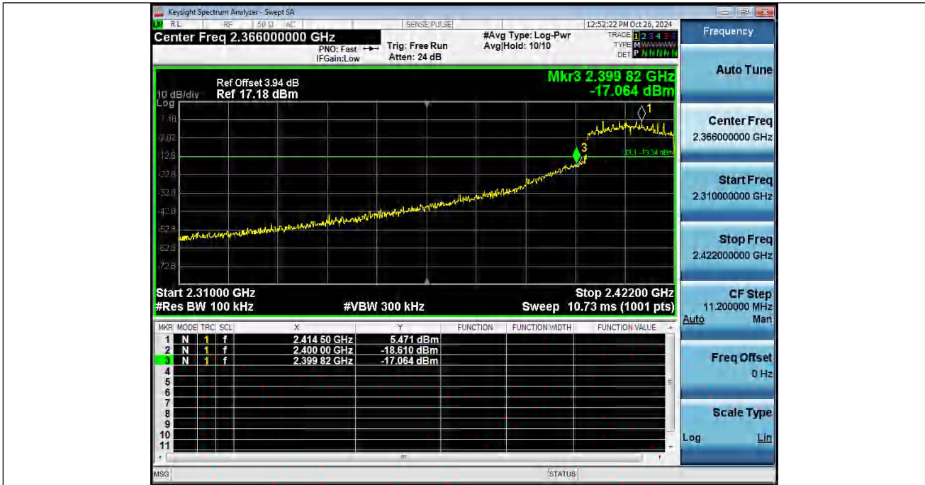
2_Bandedge_NVNT_ANT2_802_11ax(HE20)_2412
