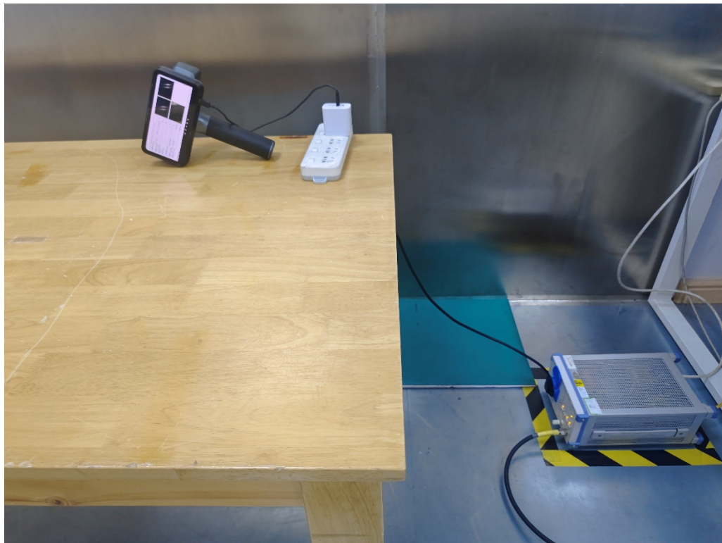
Photograph 3: Set-up photo for AC Conducted Emissions
