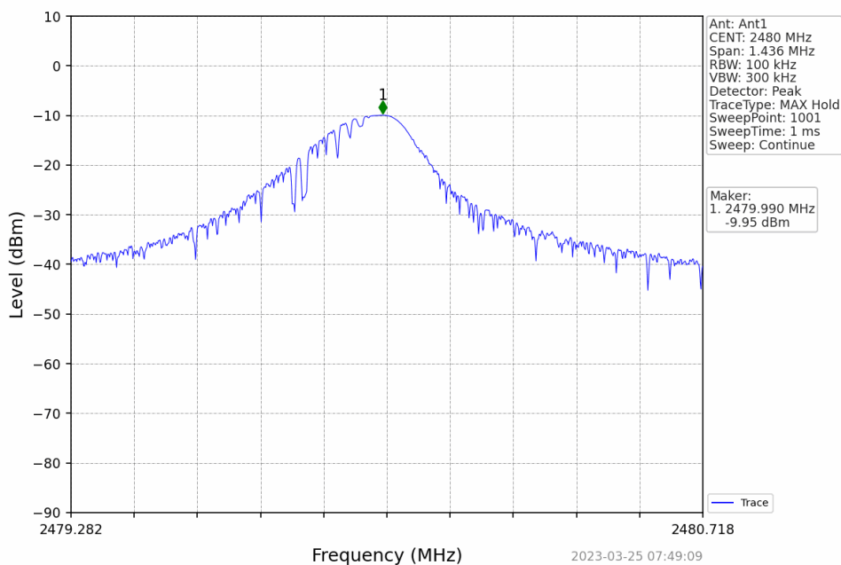
GFSK_DH5_HCH_2480MHz
