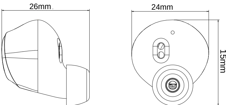
Headset
