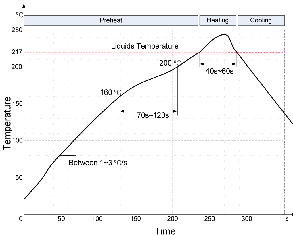
Figure 9: Reflow Soldering Thermal Profile
