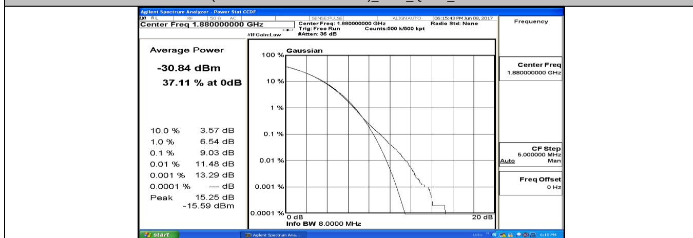
(Channel Bandwidth:20 MHz)_MCH_QPSK_1RB#49
