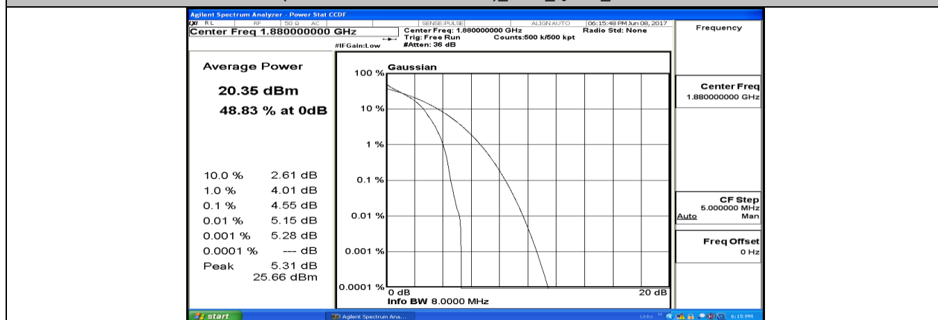
(Channel Bandwidth:20 MHz)_MCH_QPSK_1RB#99
