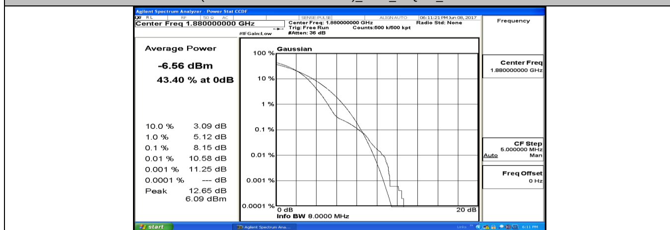
(Channel Bandwidth:15 MHz)_MCH_16QAM_1RB#37
