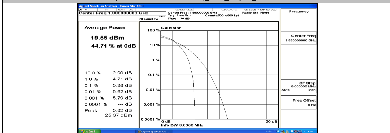
(Channel Bandwidth:15 MHz)_MCH_16QAM_1RB#74
