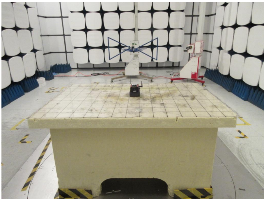
Radiation Emission L
