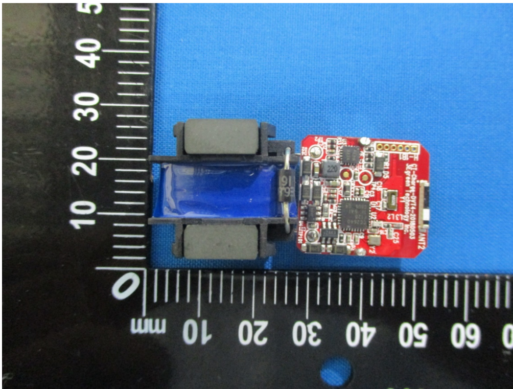
Series Model: CM00-01 EUT- Main Board Top View
