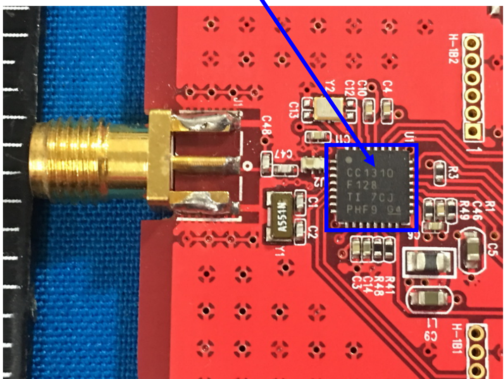
SUB 1G RF Chip IC – Top View
