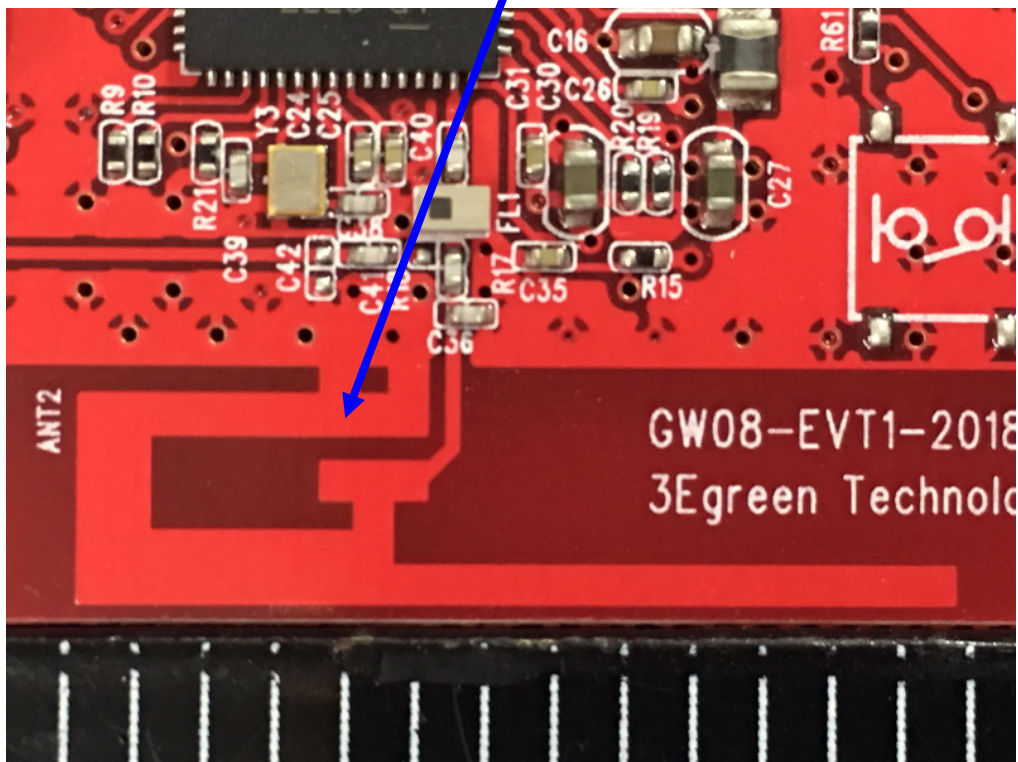
PCB Antenna – Top View
