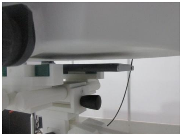
Photo 6: Body-Worn Front(10mm)
