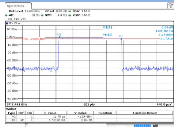
GFSK DH3
