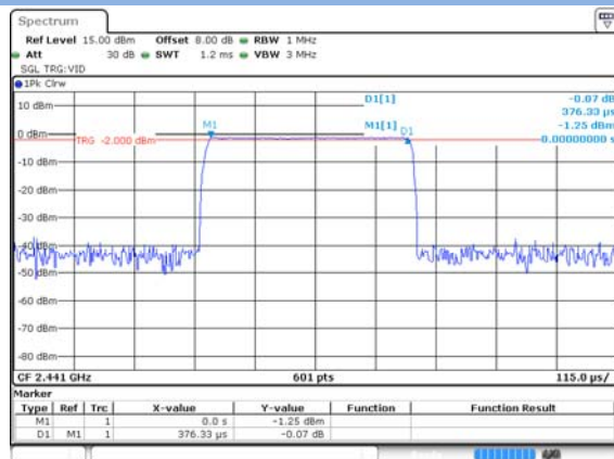
GFSK DH1
