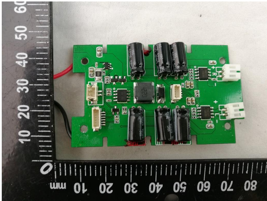
MAIN BOARD 3 FRONT VIEW
