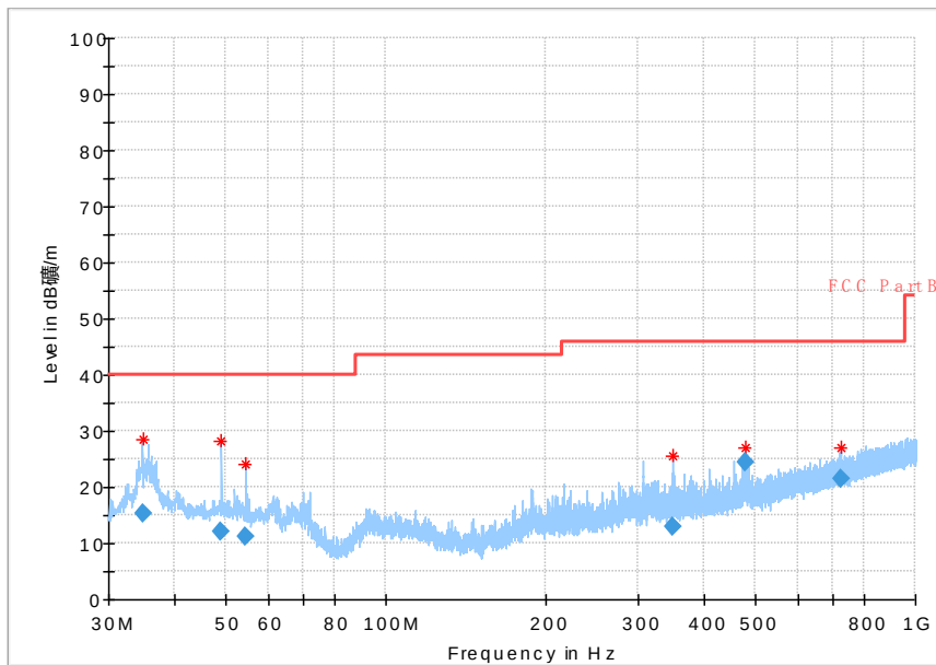
Fig.18 Radiated emission: Ch0, 30MHz~1GHz
