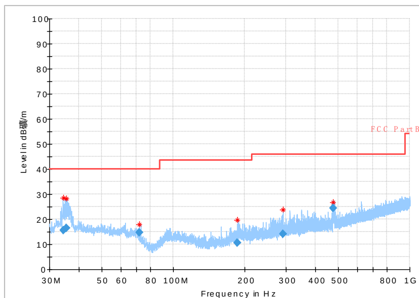
Fig.21 Radiated emission: Ch39, 30MHz~1GHz
