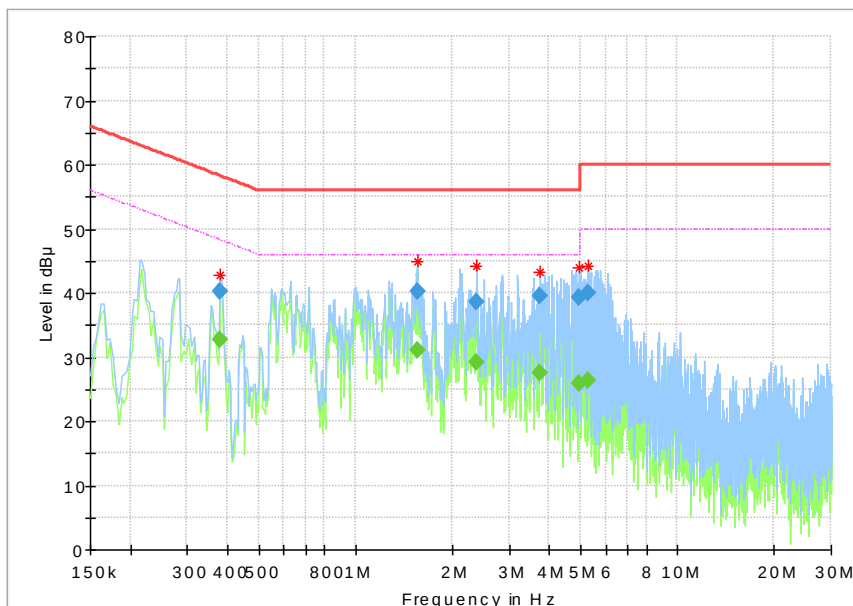
Fig.24 AC Powerline Conducted Emission
