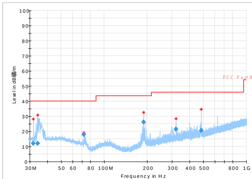
Fig.74 Radiated Spurious Emission (802.11 n-40MHz,Ch3,30MHz~1GHz)
