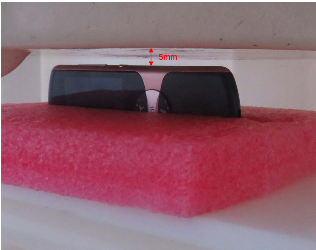
Right Edge, the distance from handset to the bottom of the Phantom is 5mm
