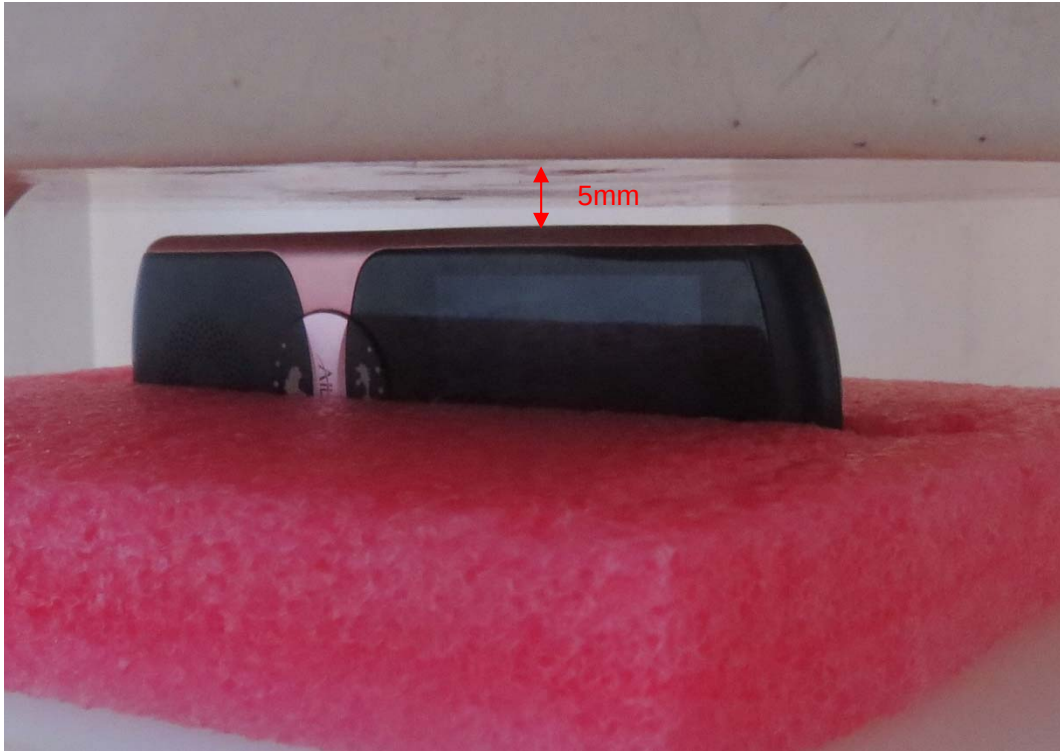
Left Edge, the distance from handset to the bottom of the Phantom is 5mm
