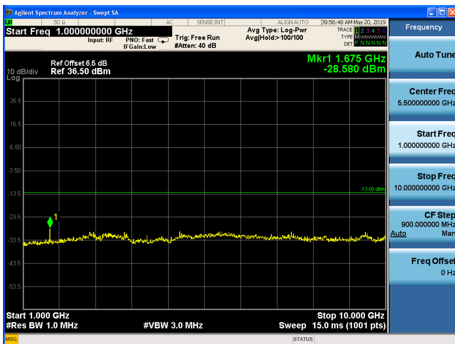
Channel 189, 1GHz~10GHz
