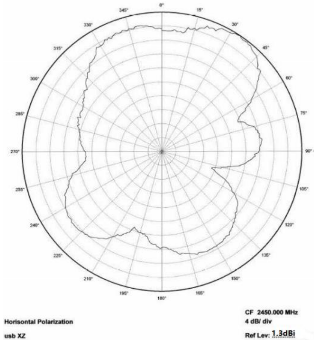
Figure 10: WLT6200 XZ Plane
