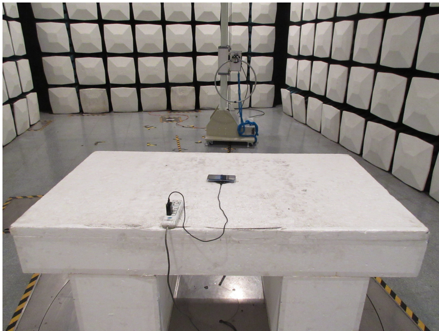
Radiated Emission Rear View (9kHz-30MHz)
