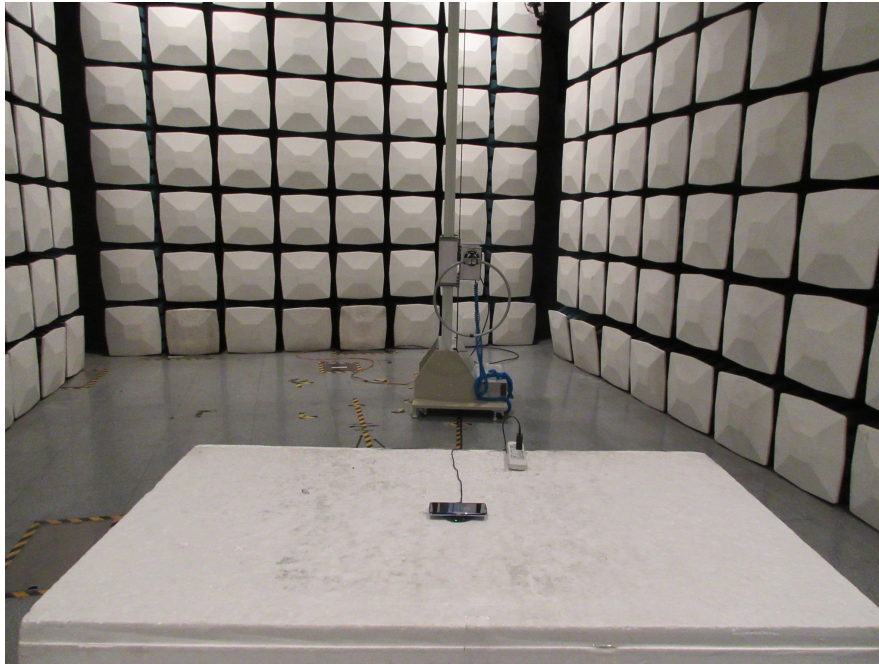
Radiated Emission Front View (9kHz-30MHz)
