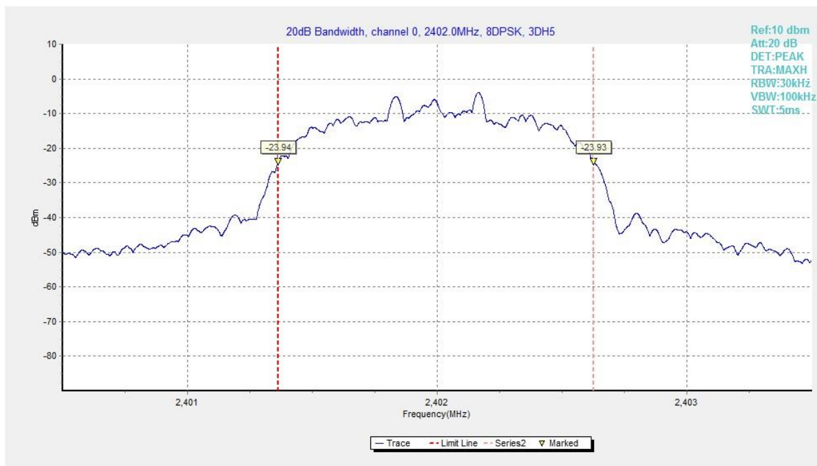
Fig. 105 20dB Bandwidth (8DPSK, Ch 0)
