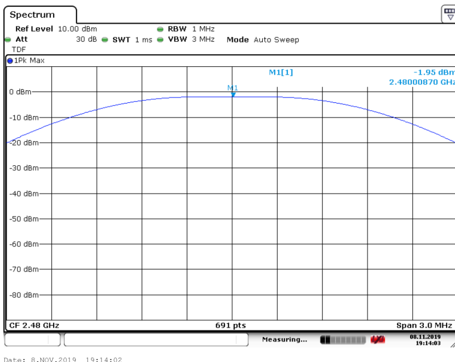
Fig.3 Maximum Peak Output Power (Ch 39)
