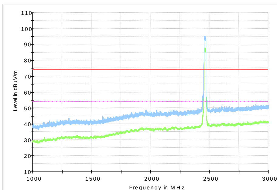
Fig.57 Radiated Spurious Emission (802.11g, Ch11, 1GHz ~3 GHz ,Horizontal Direction)
