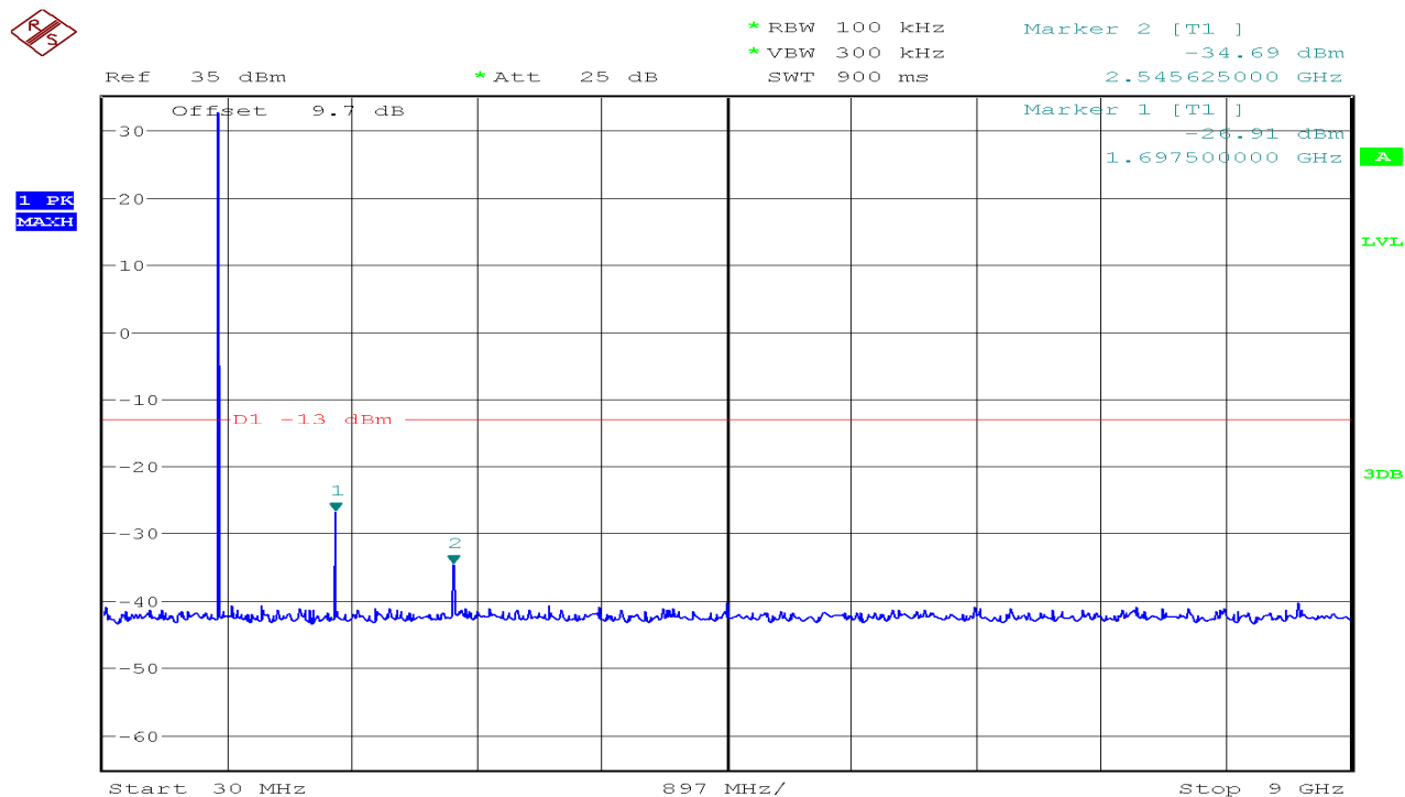
Figure 11-3: Out of Band emission at antenna terminals – GPRS CH High
