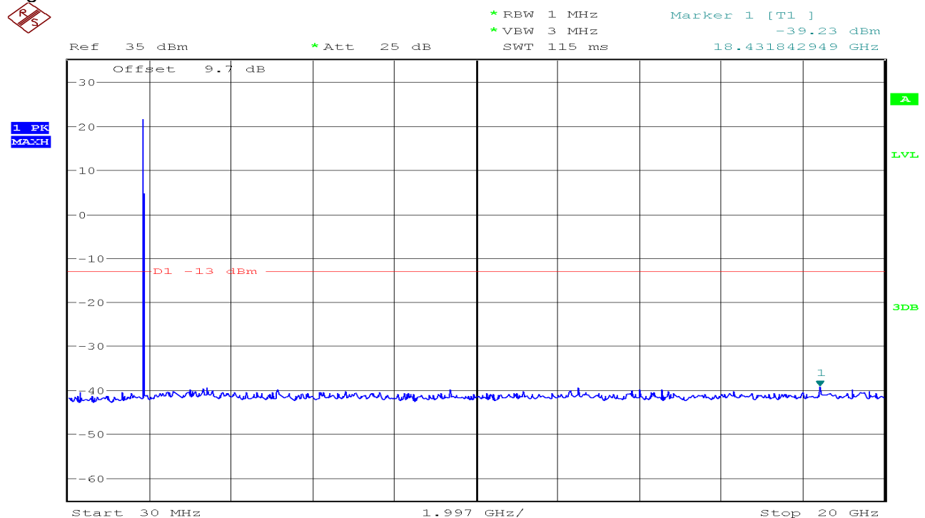
Figure 17-2: Out of Band emission at antenna terminals – HSDPA CH Mid
