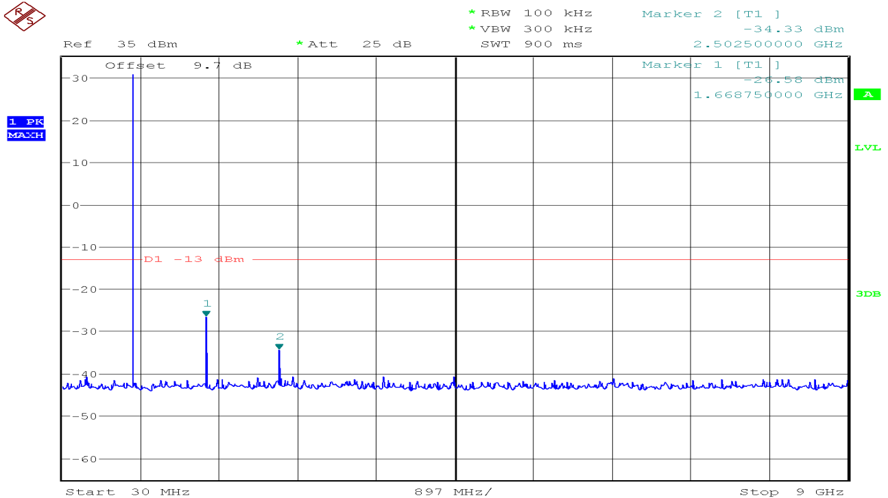
Figure 12-2: Out of Band emission at antenna terminals – EGPRS CH Mid
