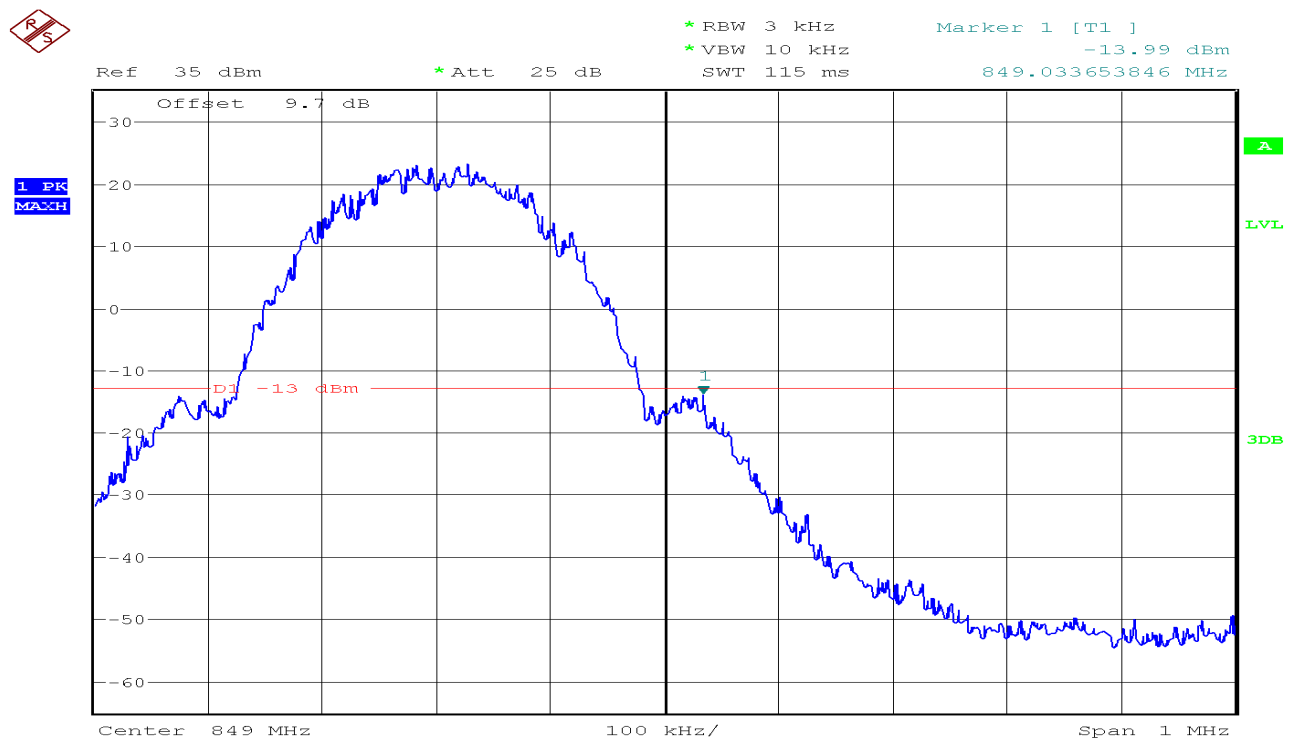
Figure 2-2: Band Edge emissions –EGPRS CH High
