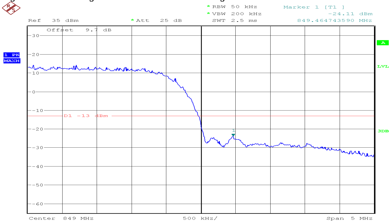
Figure 8-2: Band Edge emissions –WCDMA CH High
