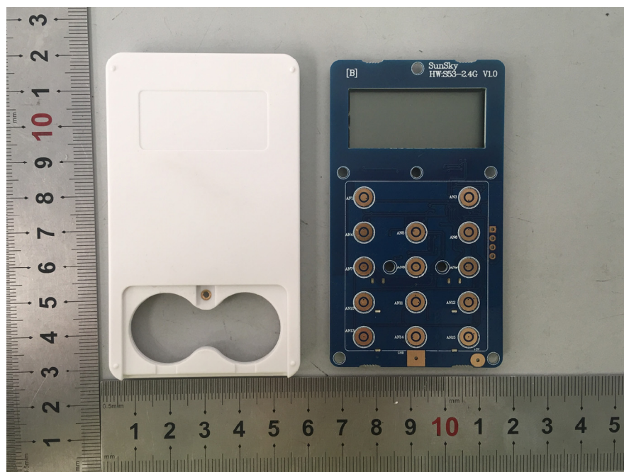
EUT – Cover off View-2(RF-09)
