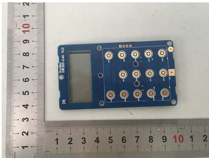
EUT – PCB Bottom View(RF-09)
