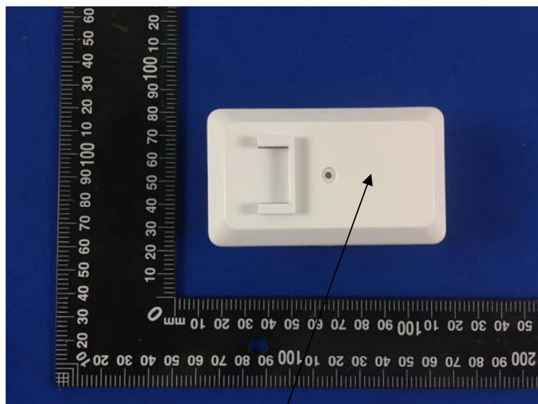
Alarm Motion Detector Model: CZ-345-PIR FCC ID: 2AMJN-CZ-345-PIR
