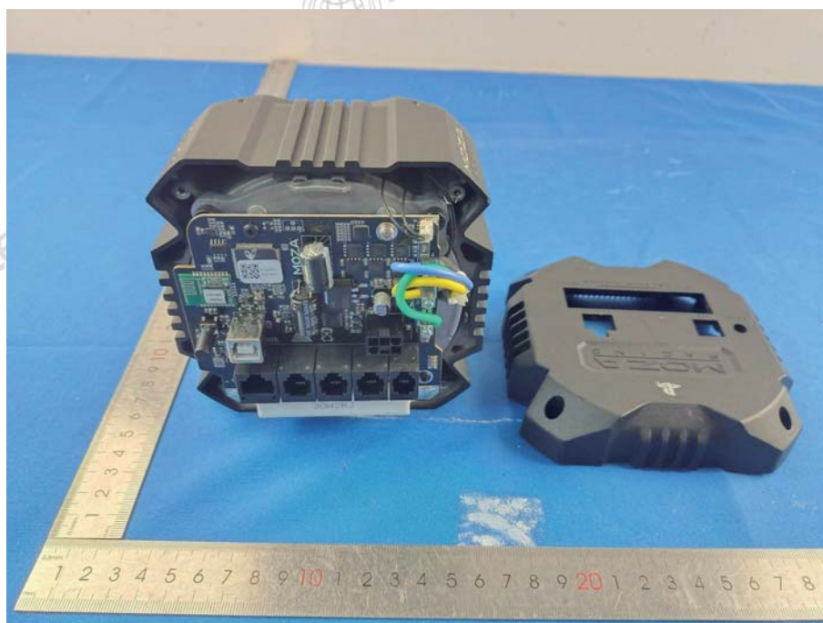
Internal R5S Pro
