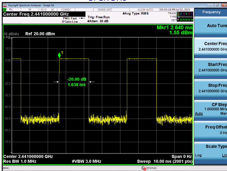
GFSK DH3
