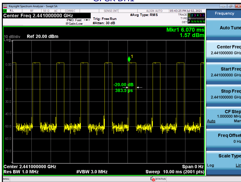
GFSK DH1
