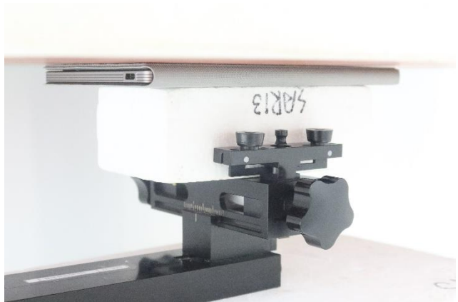
Back with Holster 1 + Pen Folding Mode at 0 mm
