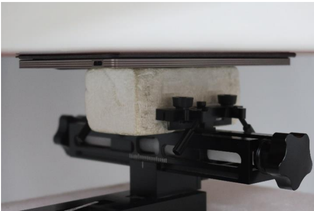
Back with Holster 2 + Pen Writing Mode at 0 mm
