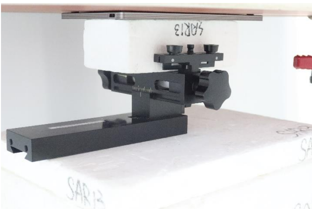
Back with Pen at 0 mm
