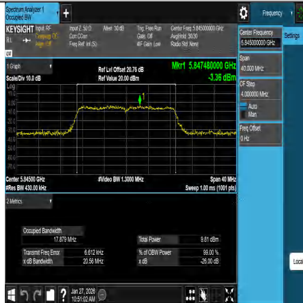
11AC20SISO-Ant1-5845
