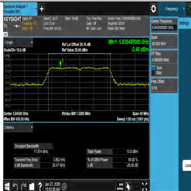
11N20SISO-Ant1-5845
