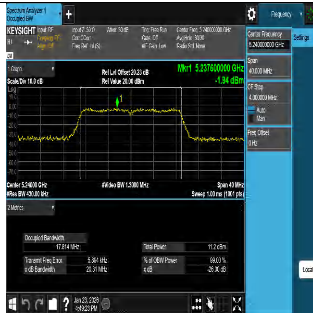
11AC20SISO-Ant1-5240
