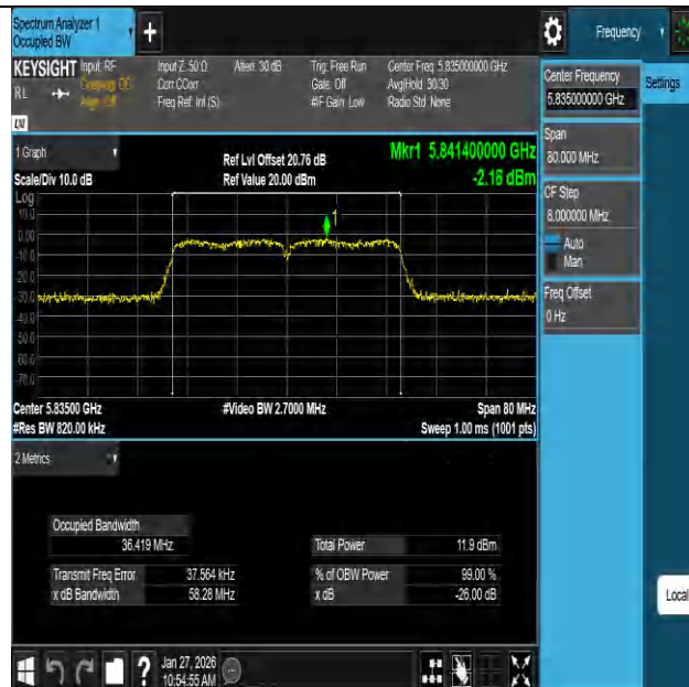
11AC40SISO-Ant1-5835
