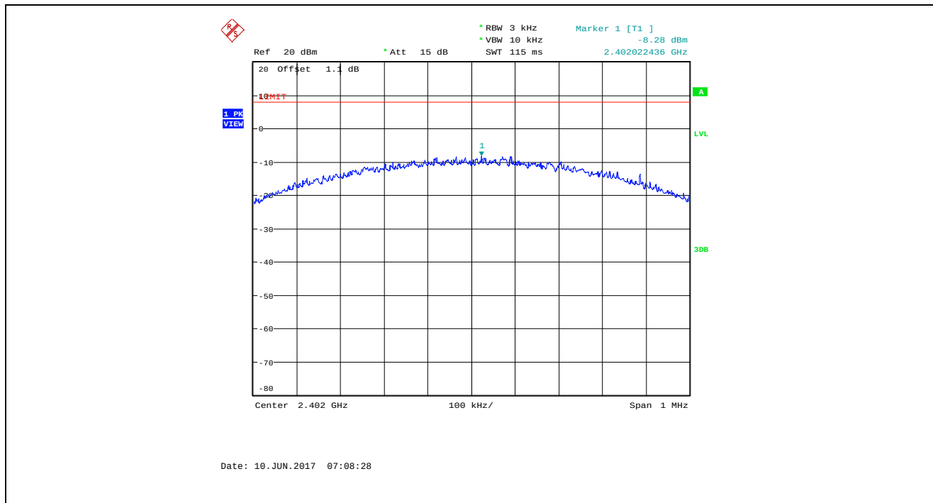
Plot 5.5.4.1. Power Spectral Density, 2402 MHz
