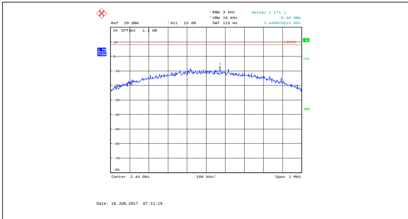
Plot 5.5.4.2. Power Spectral Density, 2440 MHz
