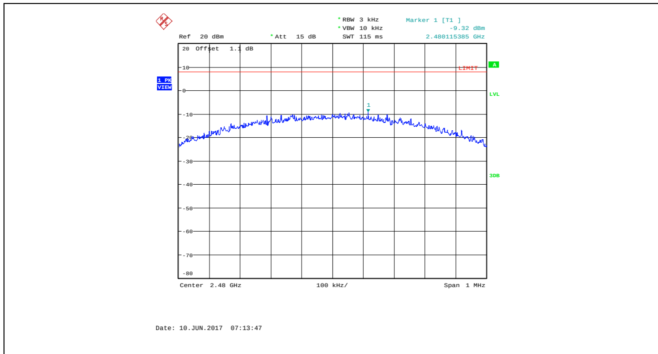
Plot 5.5.4.3. Power Spectral Density, Bandwidth 2480 MHz
