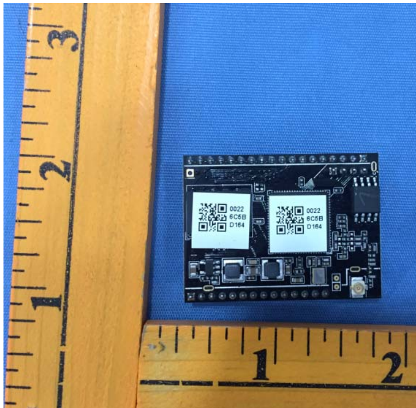
EUT – WIFI Module View
