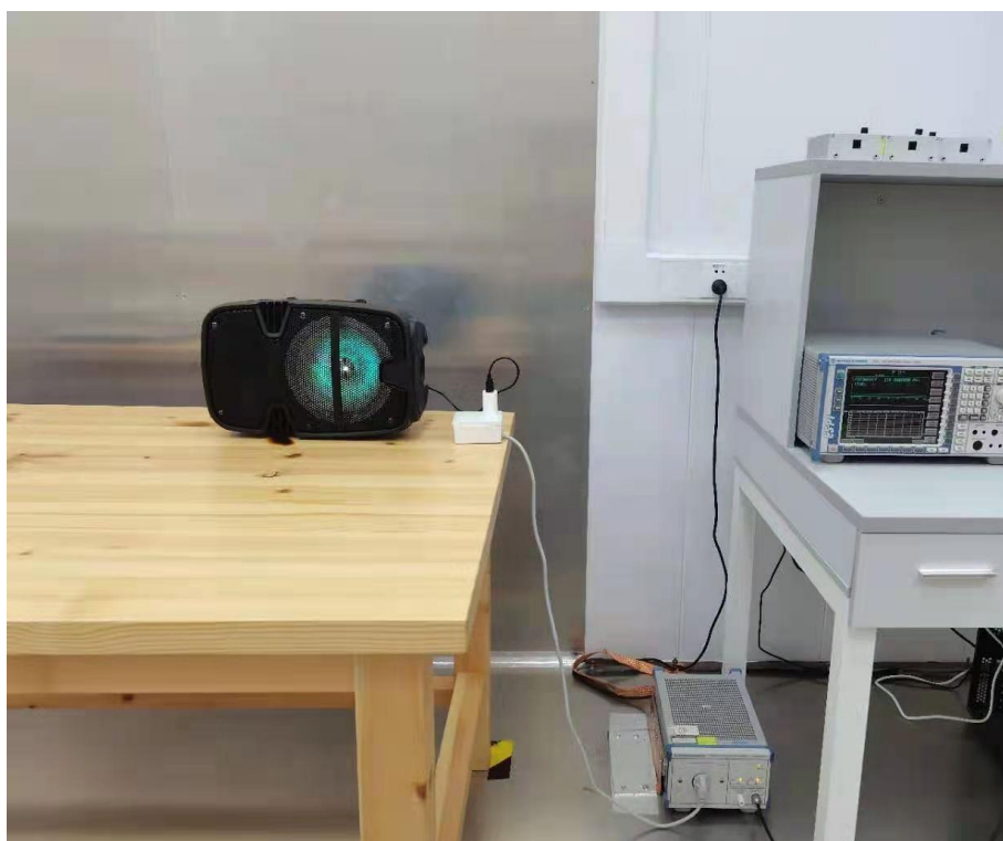
Test Setup Photo of Line Conducted Emissions Measurement
