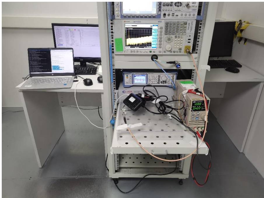
Conducted Test-WIFI 2.4G
