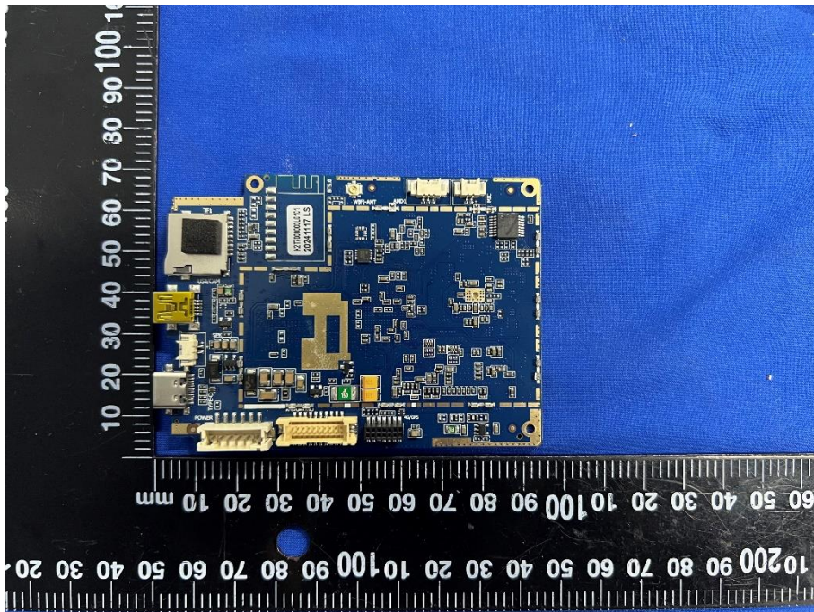
SECONDARY BOARD REAR VIEW (WITHOUT SHIELDING)
