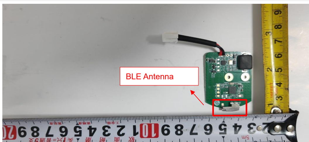
MAIN BOARD TOP VIEW
