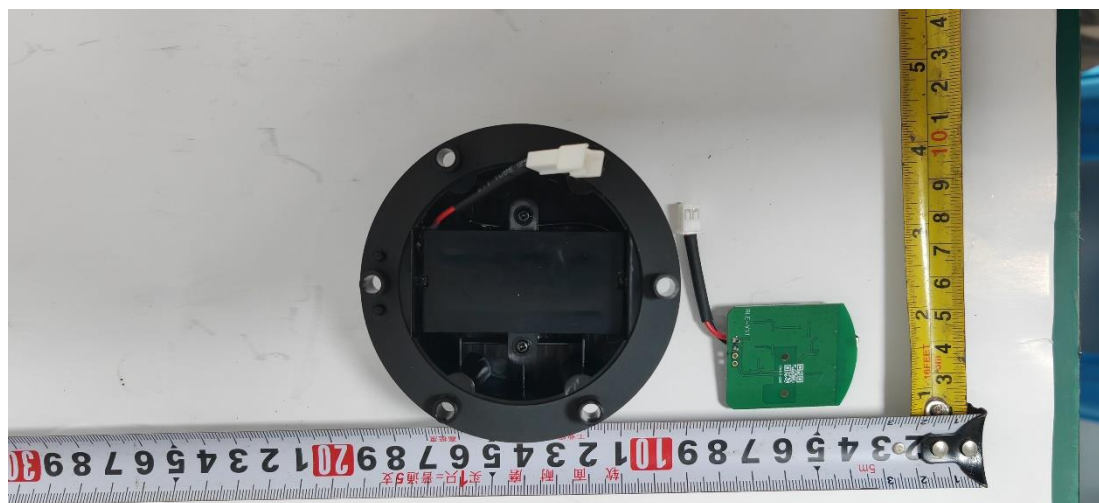
EUT UNCOVER VIEW 3
