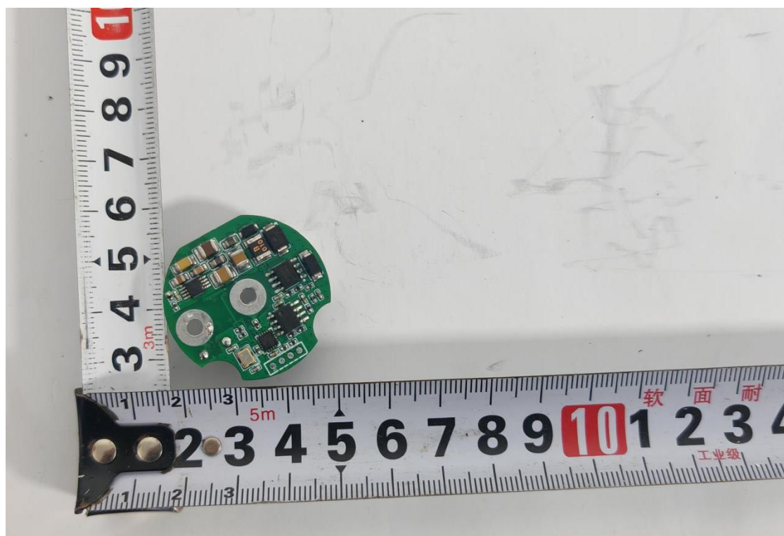
PCB BOARD TOP VIEW
