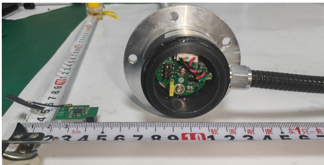
EUT UNCOVER VIEW 2
