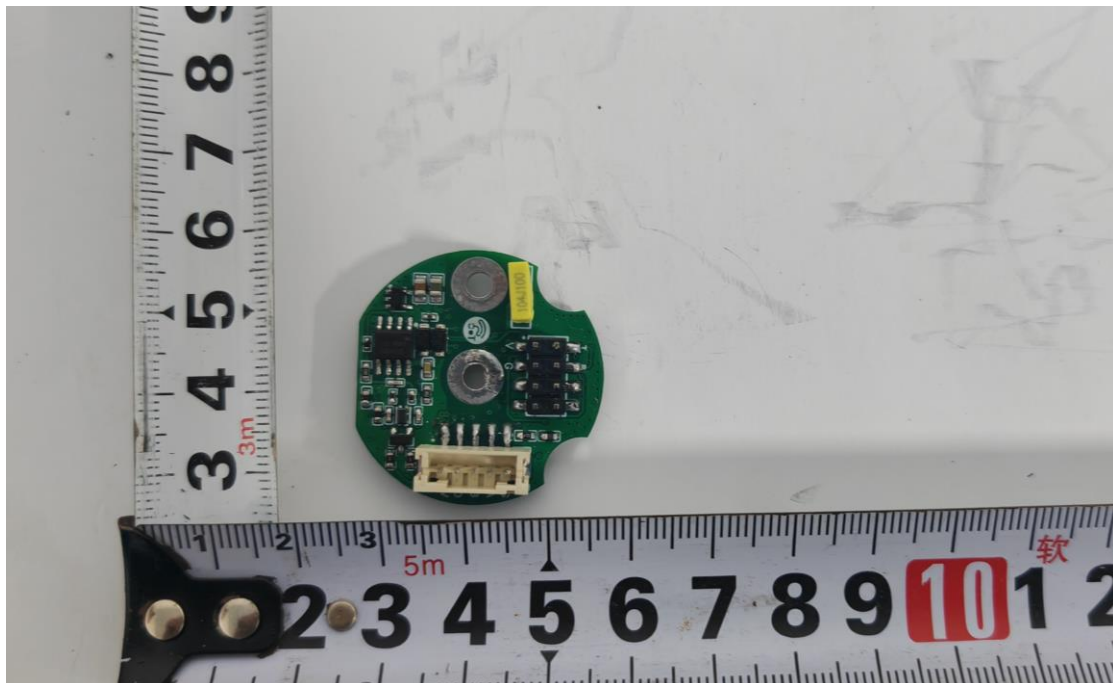
PCB BOARD REAR VIEW
