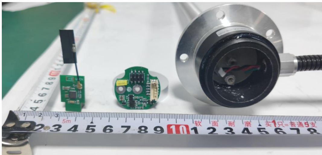
EUT UNCOVER VIEW 3
