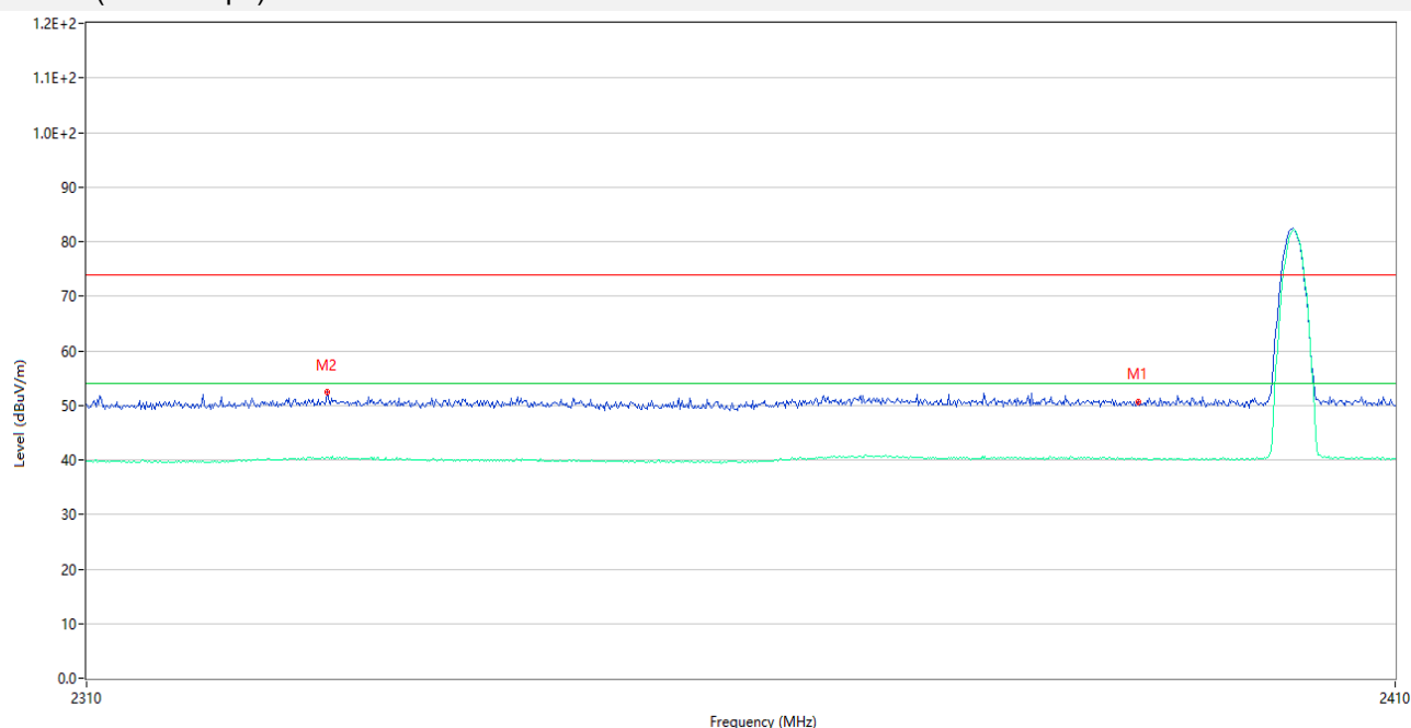
GFSK (BLE 1Mbps) LOW CHANNEL
