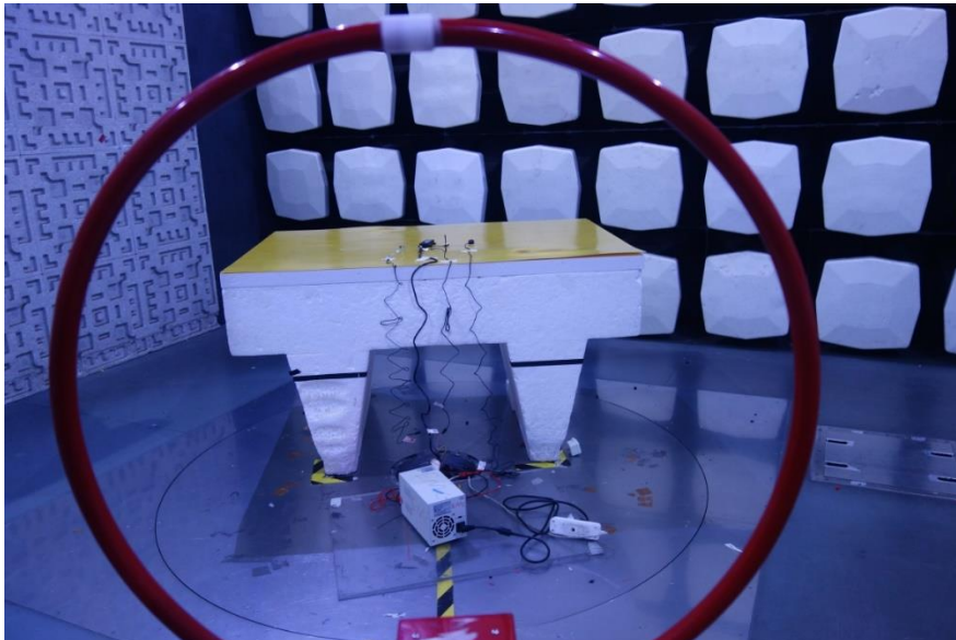
Radiated Spurious Emissions Below 1GHz
