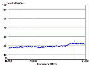
BLE_TX_CH_M_Vertical
