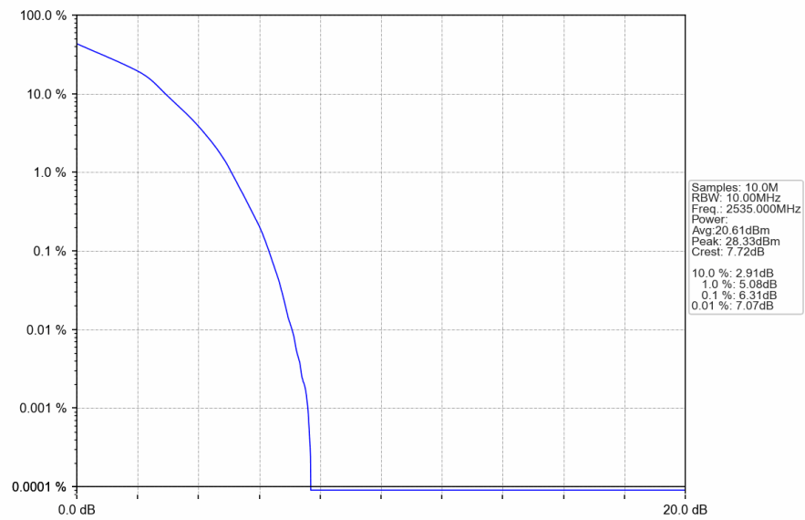
Band7_10MHz_16QAM_MCH_2535MHz_RB_27_0_NTNV
