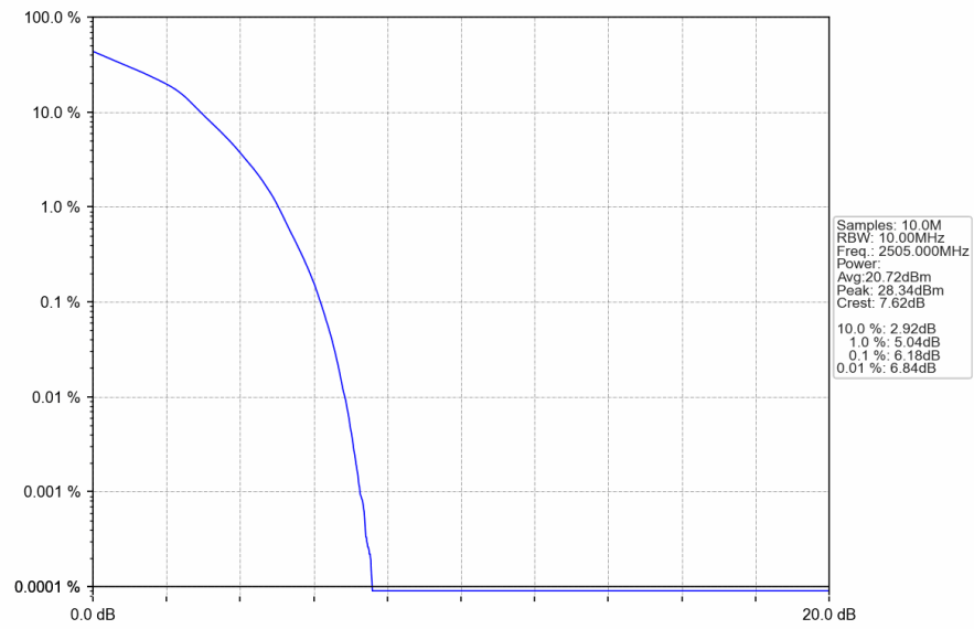
Band7 10MHz 16QAM LCH 2505MHz RB 27 0 NTN
