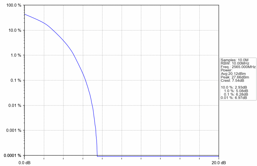
Band7_10MHz_16QAM_HCH_2565MHz_RB_27_23_NTNV
