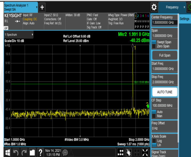
Band2-1.4MHz-QPSK-18900-1RB#0-Range2:1000~2000MHz
