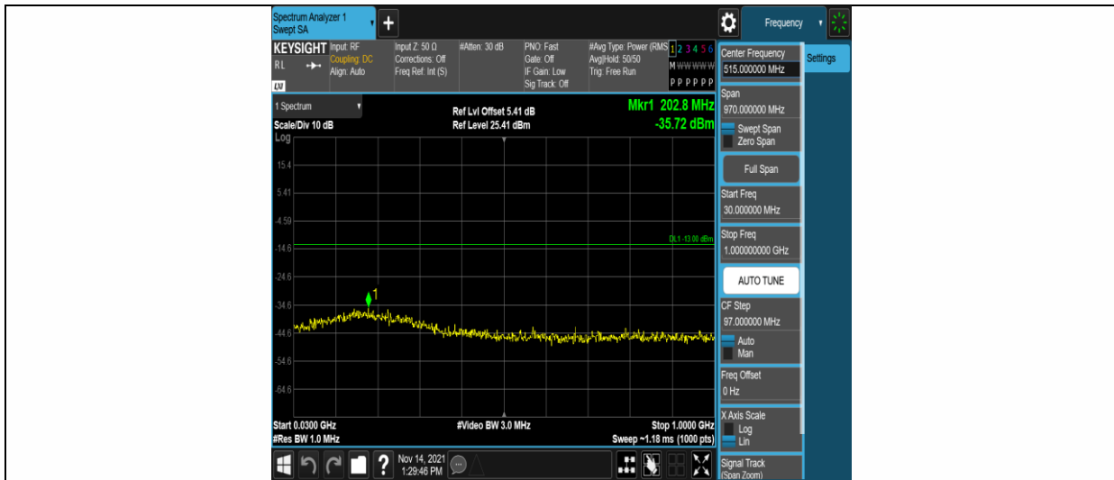
Band2-1.4MHz-QPSK-18607-1RB#0-Range1:30~1000MHz
