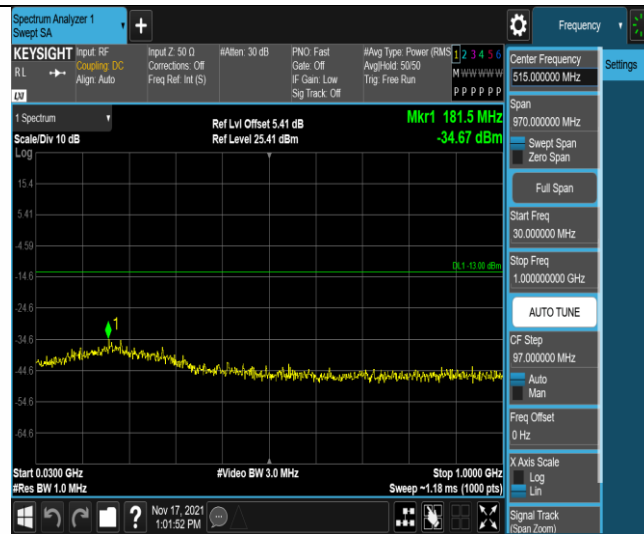
Band4-5MHz-16QAM-20175-1RB#0-Range1:30~1000MHz
