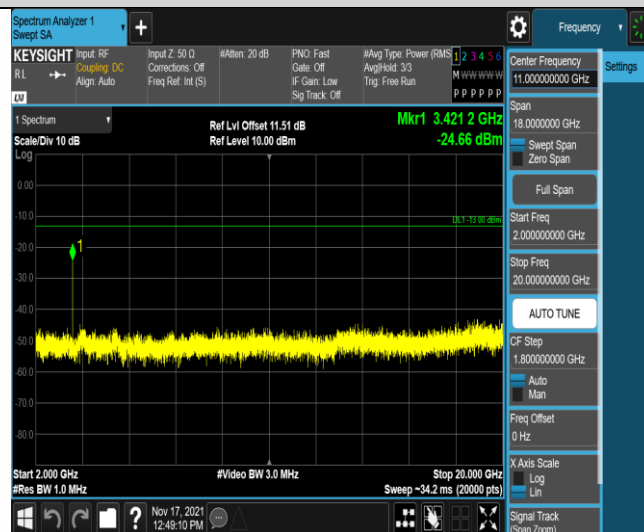
Band4-5MHz-QPSK-19975-1RB#0-Range3:2000~20000MHz
