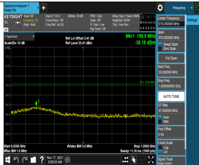
Band4-1.4MHz-16QAM-20393-1RB#0-Range1:30~1000MHz
