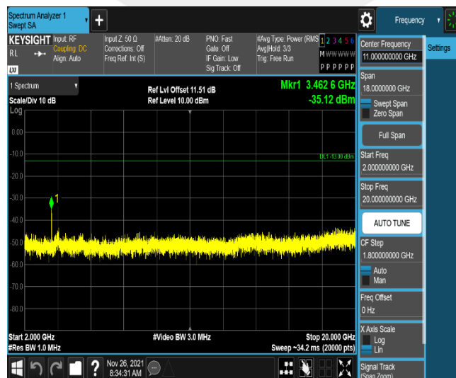
Band4-3MHz-16QAM-20175-1RB#0-Range3:2000~20000MHz
