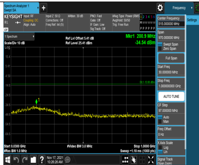
Band4-3MHz-16QAM-19965-1RB#0-Range1:30~1000MHz
