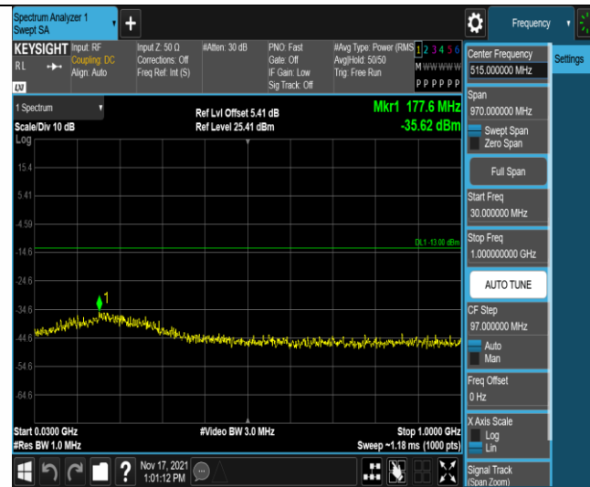
Band4-5MHz-QPSK-20175-1RB#0-Range1:30~1000MHz
