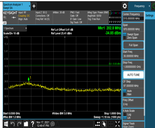
Band4-5MHz-QPSK-19975-1RB#0-Range1:30~1000MHz
