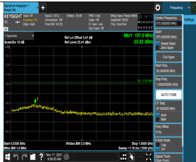
Band4-1.4MHz-16QAM-20175-1RB#0-Range1:30~1000MHz
