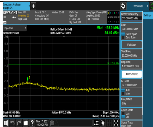
Band4-3MHz-16QAM-20175-1RB#0-Range1:30~1000MHz
