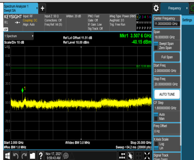
Band4-1.4MHz-16QAM-20393-1RB#0-Range3:2000~20000MHz
