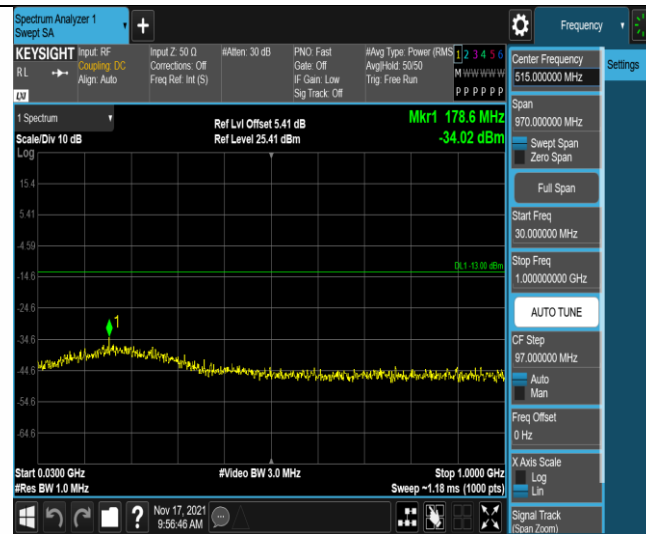
Band4-1.4MHz-16QAM-19957-1RB#0-Range1:30~1000MHz
