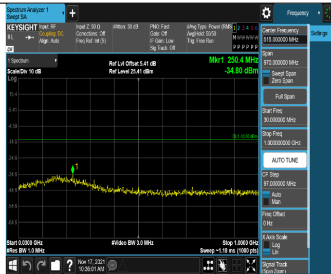
Band4-3MHz-16QAM-20385-1RB#0-Range1:30~1000MHz
