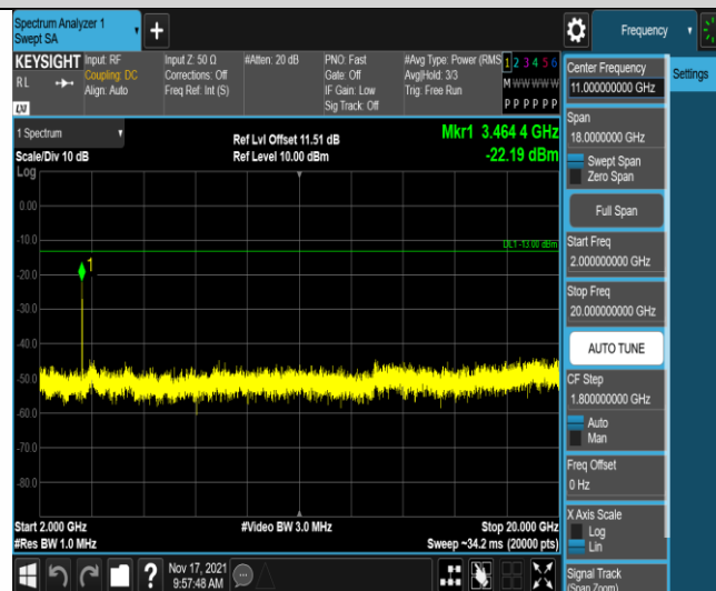
Band4-1.4MHz-QPSK-20175-1RB#0-Range3:2000~20000MHz
