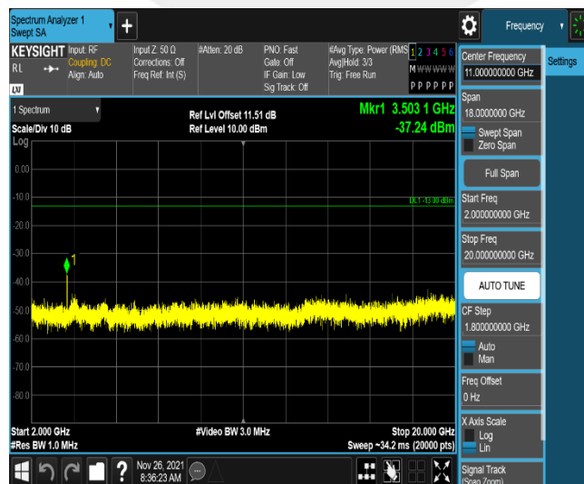
Band4-3MHz-16QAM-20385-1RB#0-Range3:2000~20000MHz
