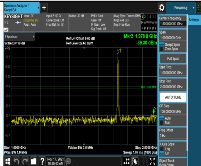
Band4-3MHz-16QAM-20175-1RB#0-Range2:1000~2000MHz
