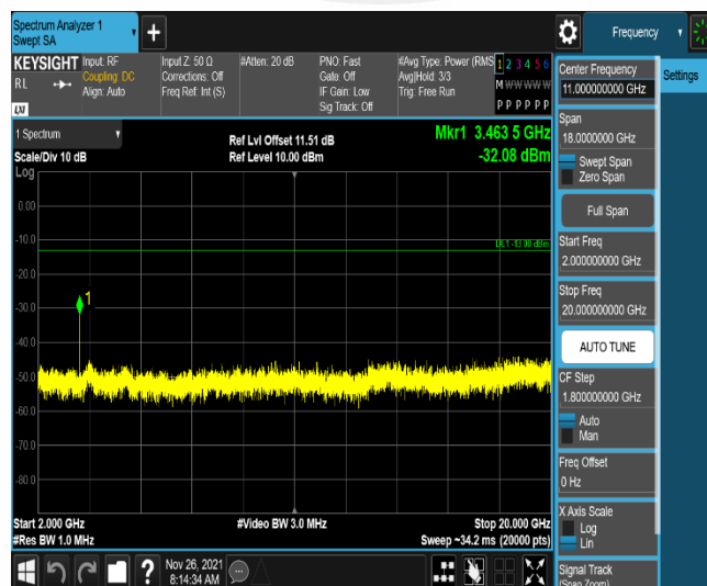
Band4-5MHz-16QAM-20175-1RB#0-Range3:2000~20000MHz
