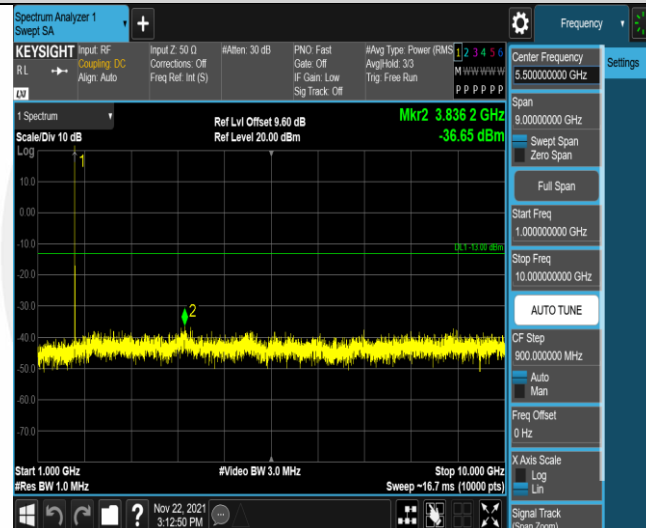
Band66-1.4MHz-QPSK-131979-1RB#0-Range2:1000~10000MHz
