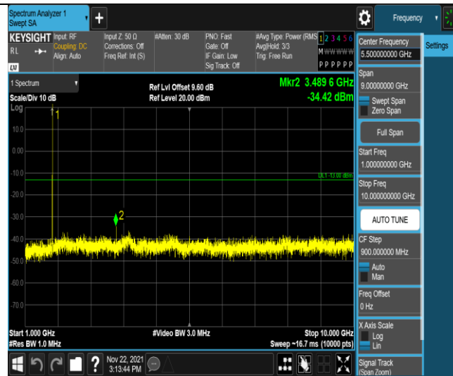
Band66-1.4MHz-QPSK-132322-1RB#0-Range2:1000~10000MHz
