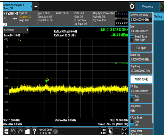
Band66-1.4MHz-16QAM-132322-1RB#0-Range2:1000~10000MHz
