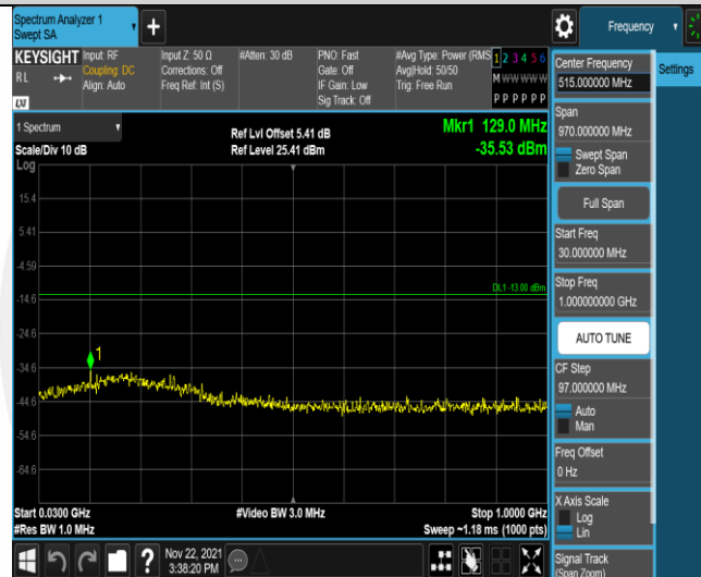
Band66-3MHz-QPSK-132657-1RB#0-Range1:30~1000MHz
