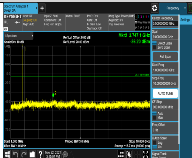
Band66-1.4MHz-16QAM-132665-1RB#0-Range2:1000~10000MHz
