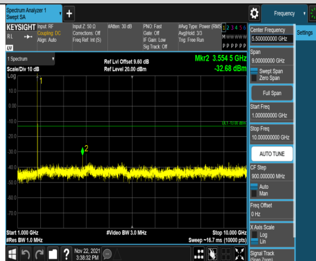
Band66-3MHz-QPSK-132657-1RB#0-Range2:1000~10000MHz
