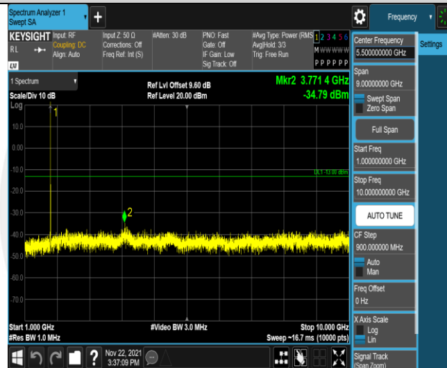
Band66-3MHz-16QAM-131987-1RB#0-Range2:1000~10000MHz
