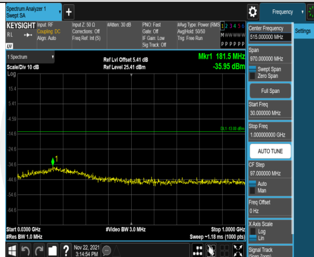
Band66-1.4MHz-16QAM-132665-1RB#0-Range1:30~1000MHz
