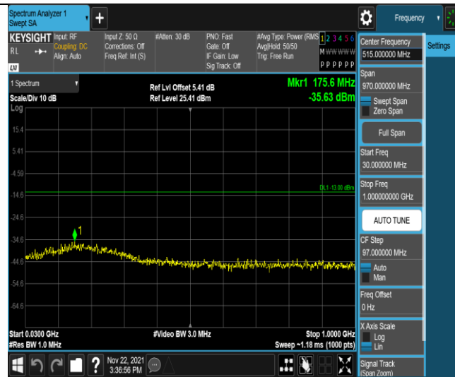
Band66-3MHz-16QAM-131987-1RB#0-Range1:30~1000MHz
