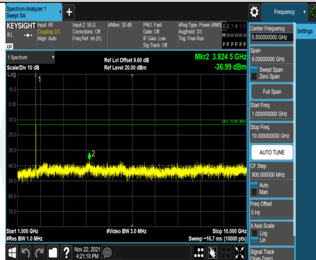
Band66-5MHz-QPSK-131997-1RB#0-Range2:1000~10000MHz
