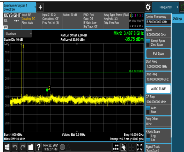
Band66-3MHz-QPSK-132322-1RB#0-Range2:1000~10000MHz
