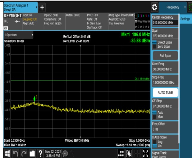
Band66-3MHz-16QAM-132657-1RB#0-Range1:30~1000MHz
