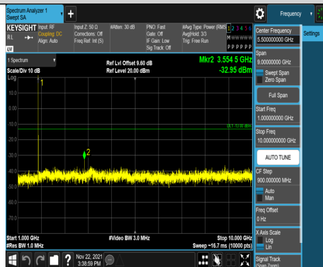
Band66-3MHz-16QAM-132657-1RB#0-Range2:1000~10000MHz
