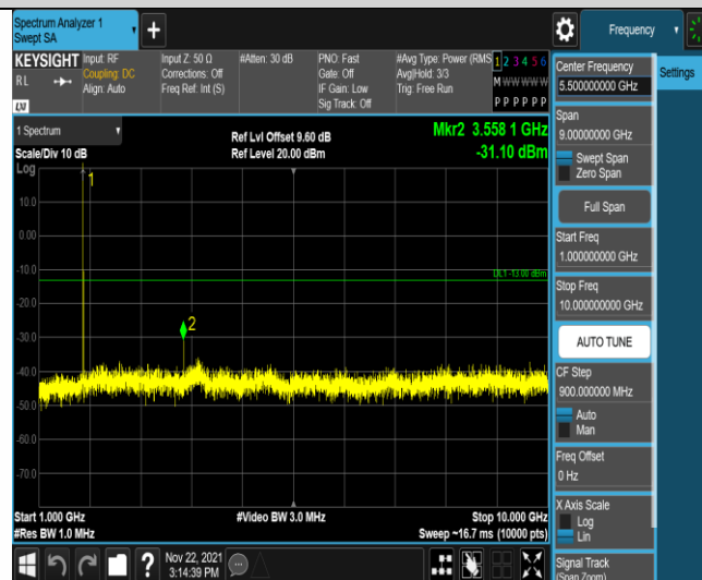
Band66-1.4MHz-QPSK-132665-1RB#0-Range2:1000~10000MHz
