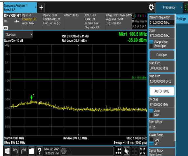
Band66-3MHz-QPSK-131987-1RB#0-Range1:30~1000MHz
