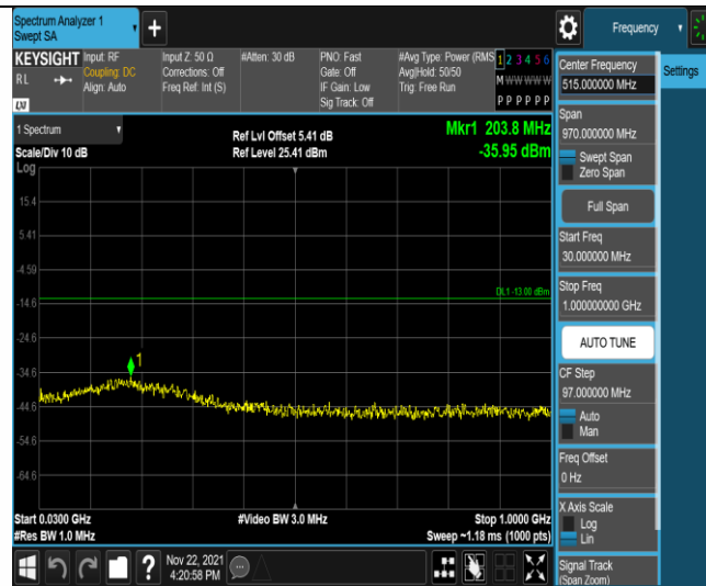
Band66-5MHz-QPSK-131997-1RB#0-Range1:30~1000MHz
