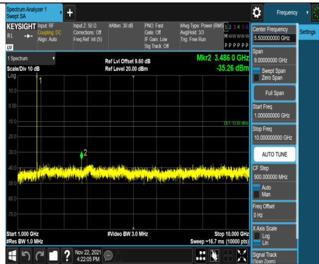
Band66-5MHz-QPSK-132322-1RB#0-Range2:1000~10000MHz
