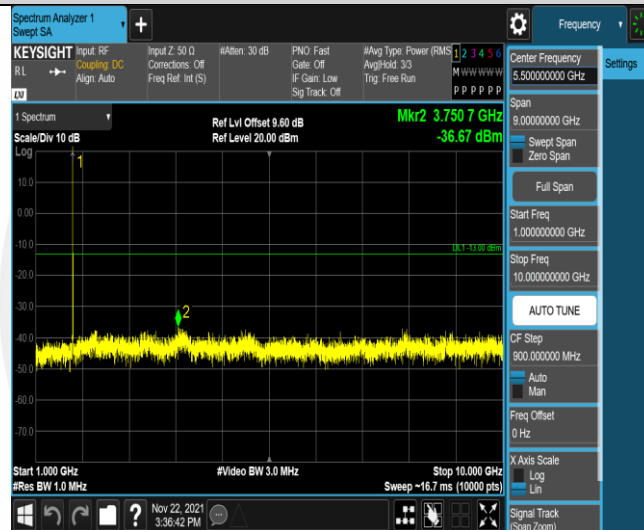
Band66-3MHz-QPSK-131987-1RB#0-Range2:1000~10000MHz
