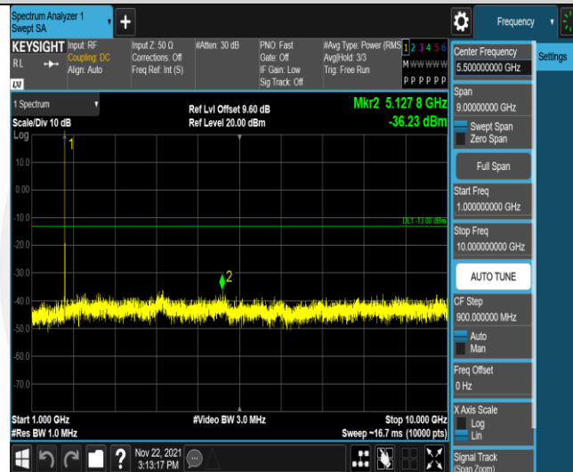
Band66-1.4MHz-16QAM-131979-1RB#0-Range2:1000~10000MHz
