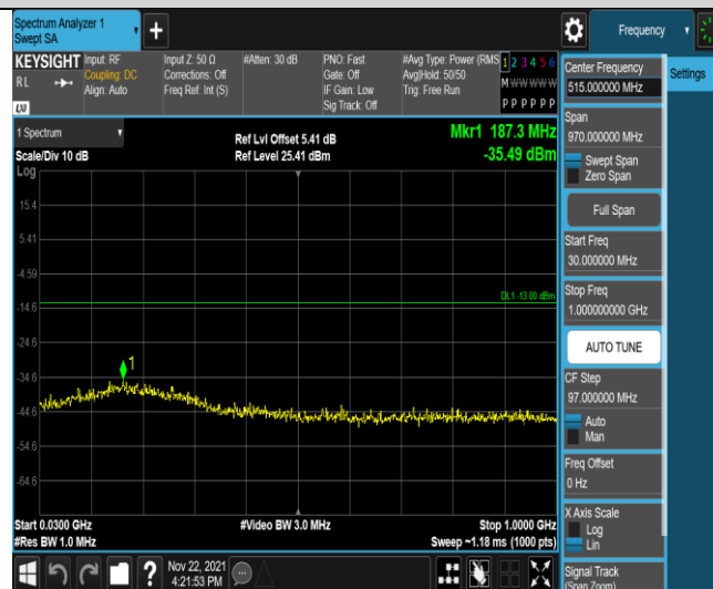
Band66-5MHz-QPSK-132322-1RB#0-Range1:30~1000MHz
