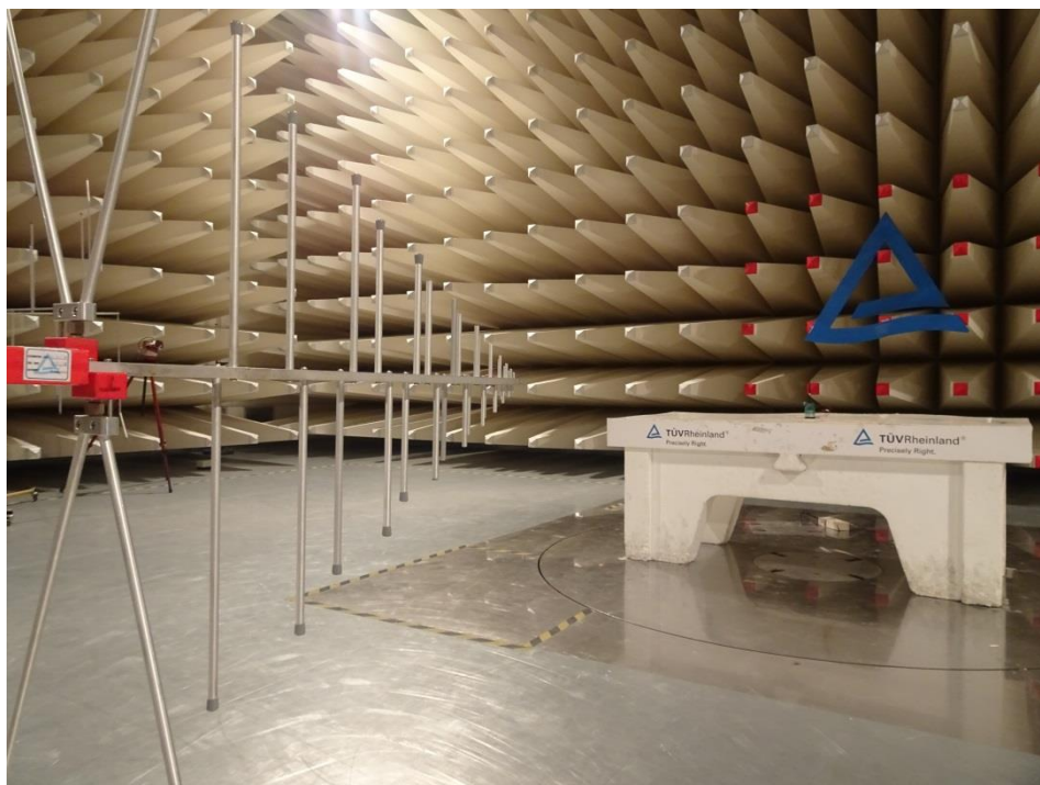
Vertical Polarization Setup Photo – 30 MHz – 1 GHz
