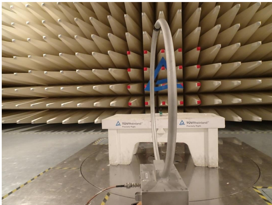
Perpendicular Polarization Setup Photo - 9 kHz – 30 MHz
