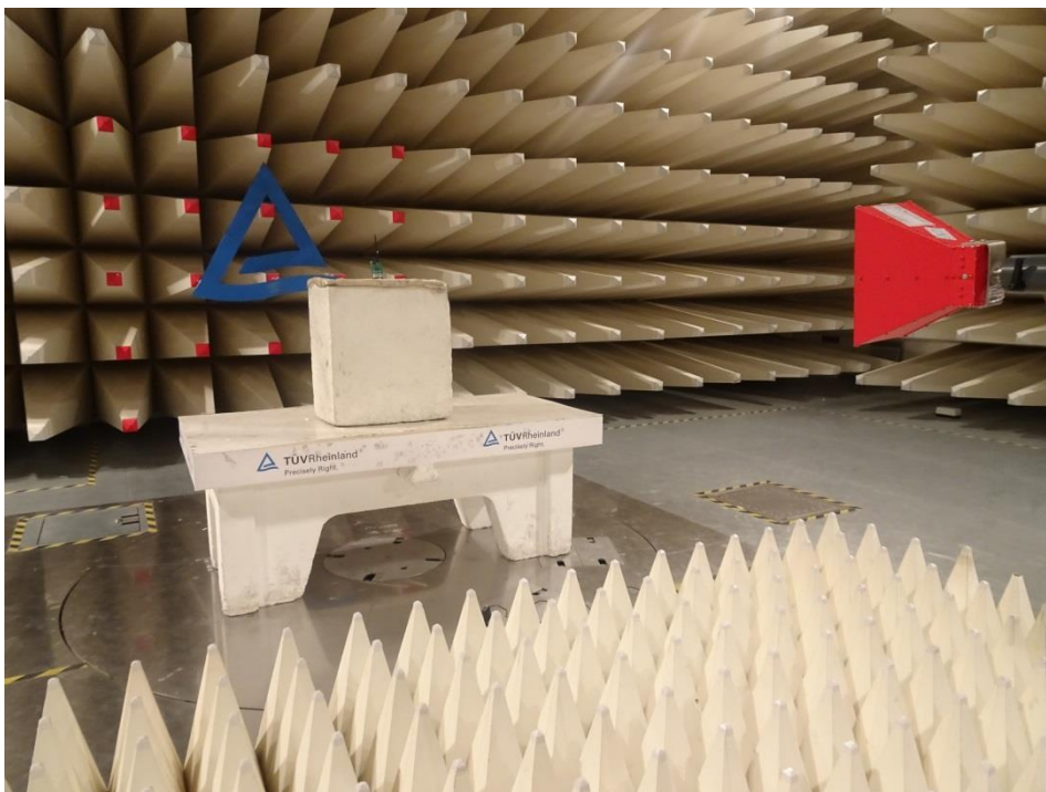
Horizontal Polarization Setup Photo - 1 GHz- 18 GHz
