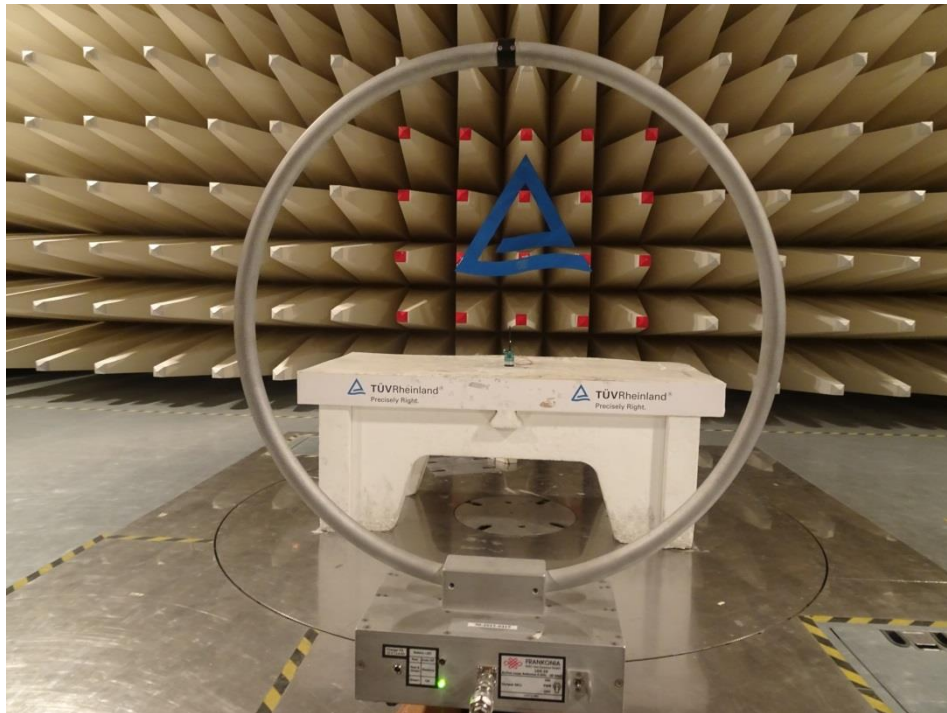
Parallel Polarization Setup Photo - 9 kHz – 30 MHz
