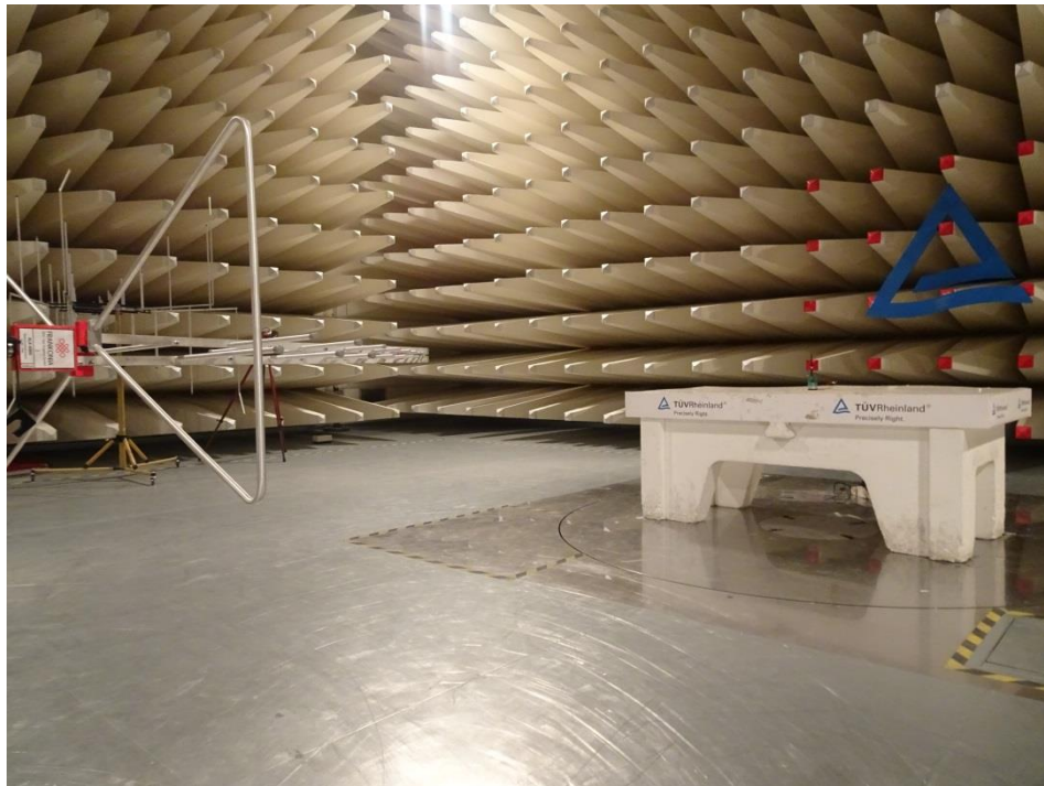
Horizontal Polarization Setup Photo – 30 MHz – 1 GHz
