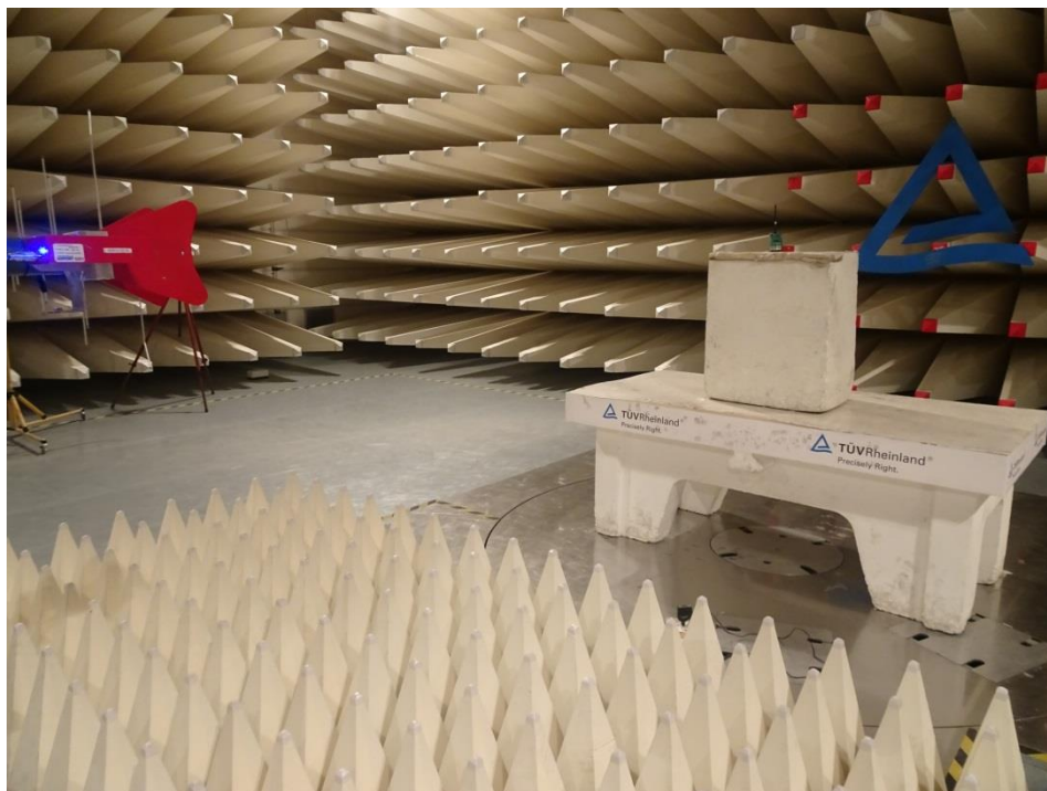
Horizontal Polarization Setup Photo - 18 GHz – 26.5 GHz
